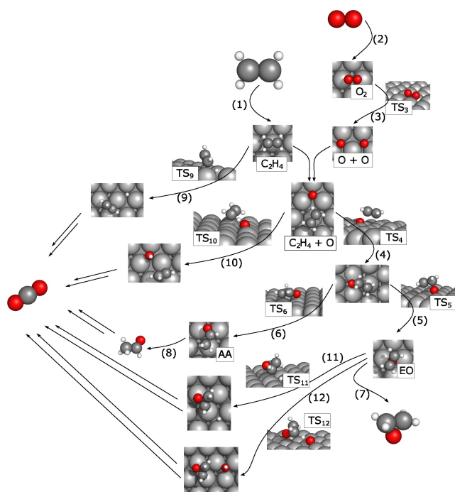
Figure 1. Scheme of the reaction mechanism on Ag(111). The reactions are numbered as in the main text. The mechanism on other investigated surfaces is analogous.
