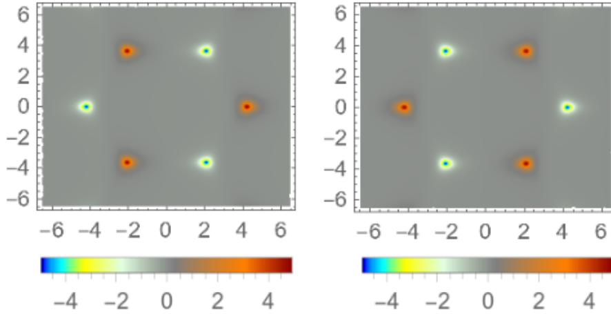
FIGURE 2.7. Berry curvatures \Omega_{n\sigma}^z for the twofold degenerate bands E_\pm with modes \sigma = \uparrow, \downarrow in the first BZ. Left: \Omega_{\pm, \downarrow}^z , right: \Omega_{\pm, \uparrow}^z . Summing over \sigma results in the vanishing Berry curvature \Omega_n^z(\vec{k}) = 0 of band n .
