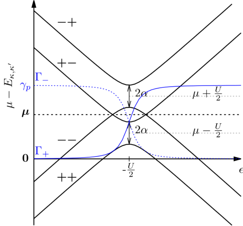
FIGURE 3.4. Addition energies E_{\kappa, \kappa'} for adding a particle (e) or a hole (h) from the metal to the quantum dot and coupling rates \Gamma_{\pm} with \eta\tau = \pm (blue lines) between the metal and the quantum dot in dependence of gate voltage \epsilon . The E_{\kappa, \kappa'} are given relative to the chemical potential. U denotes the Coulomb interaction and \alpha the superconducting coupling strength.
