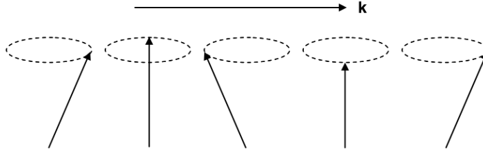
FIGURE 2.1. Propagation of a spin wave through a linear chain of spins, with spins on sites i, i' precessing at phase difference \Delta\phi = i\vec{k}(\vec{R}_i - \vec{R}_{i'}) , taken from [23].
