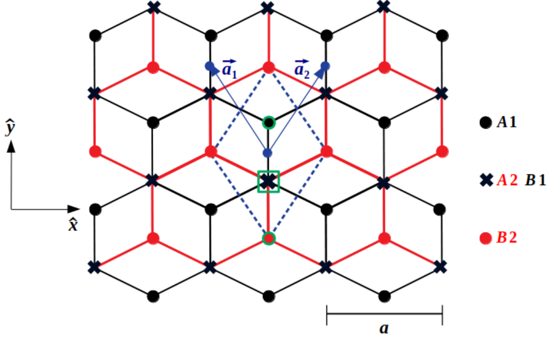
FIGURE 2.2. A bilayer with AB -stacking as, for example, in bulk \text{BiI}_3 crystals. The bottom layer (label 1) is indicated in black color and the top layer (label 2) in red. The two sublattices A and B of atoms within a layer are represented by crosses and dots, see the legend. The crosses refer to dimers. A dimer contains one atom of each layer coupled to each other providing the only type of coupling between the two layers. The primitive unit cell (dashed blue lines) with basis vectors \vec{a}_1, \vec{a}_2 spans the lattice. It contains four atoms marked in green: A 1 (green-rimmed black dot), B 2 (red-green) and the dimer pair B 1- A 2 (black-green cross).
