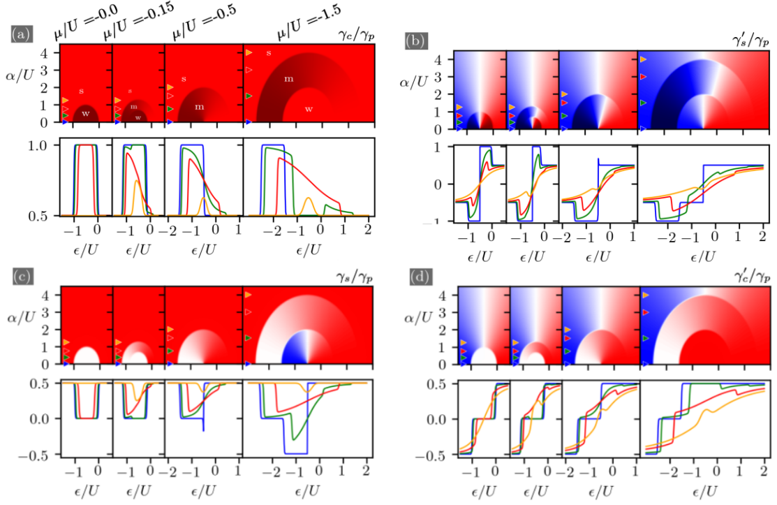
FIGURE 5.3. Duality invariants for T = 0.02U as function of the gate-voltage \epsilon = \delta - U/2 and induced pairing \alpha . All color plots use the same color scale, positions of horizontal line cuts are indicated by arrows. The semi-circles centered at \epsilon = -U/2 with radii |2\mu \pm U| [Eq. 5.11] separate the regimes of weak (w), moderate (m) and strong (s) pairing as indicated in panel (a). For further explanations see the text.
