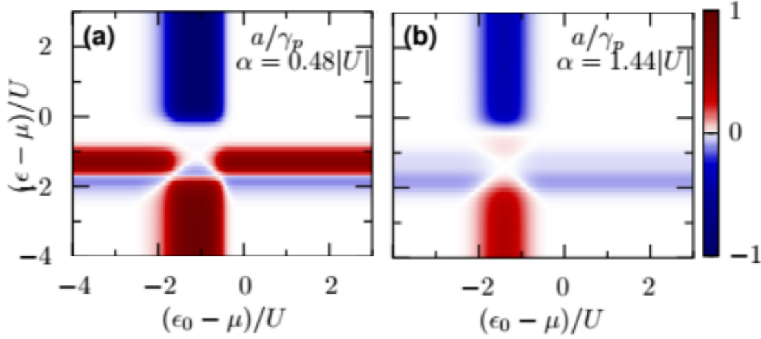
FIGURE 6.2. Charge amplitudes a after a slow switch at chemical potential \mu = 1.2U and temperature T = 0.1|U| (a) for weak pairing \alpha = 0.48|U| and (b) for strong pairing \alpha = 1.44|U| .
