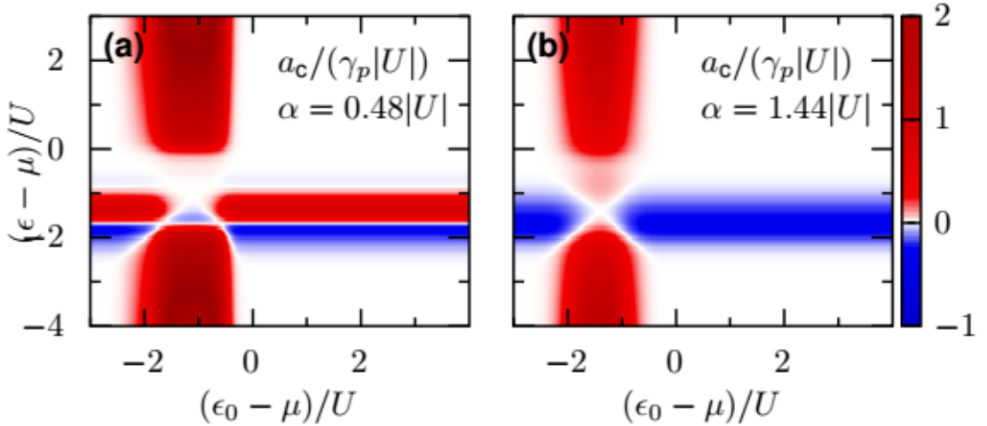
FIGURE 6.3. Charge amplitudes a_c of the heat current after a slow switch at chemical potential \mu = 1.2U and temperature T = 0.1|U| (a) for weak pairing \alpha = 0.48|U| and (b) for strong pairing \alpha = 1.44|U| .
