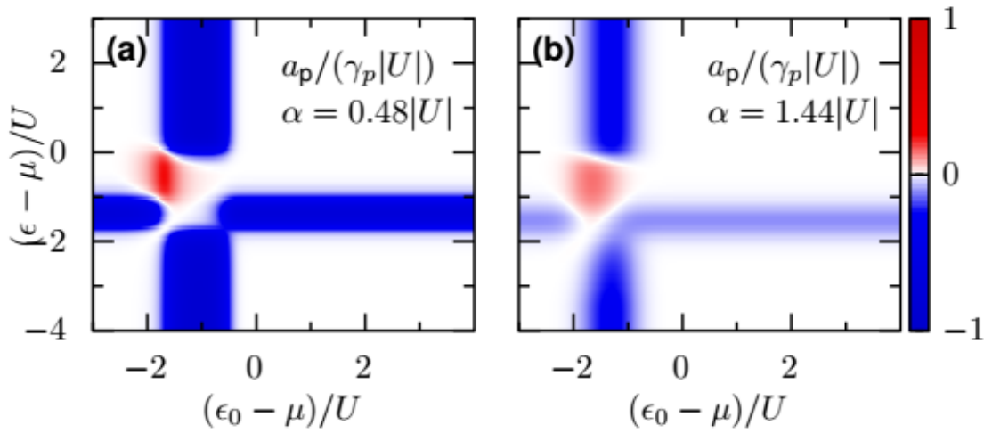
FIGURE 6.4. Parity amplitudes a_p of the heat current after a slow switch at chemical potential \mu = 1.2U and temperature T = 0.1|U| (a) for weak pairing \alpha = 0.48|U| and (b) for strong pairing \alpha = 1.44|U| .
