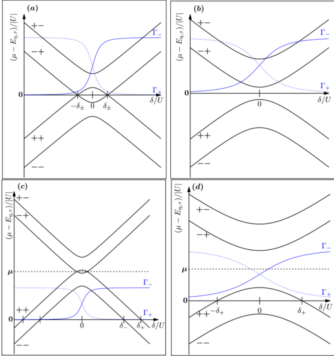
FIGURE 6.1. Schematic overview of zero temperature energy thresholds \mu - E_{\eta,\tau} (Table 6.1) for the cases of (a) \mu = 0 and weak pairing \alpha , (b) strong \alpha , (c) \mu > 0 and weak \alpha and (d) moderate \alpha . \delta_{\pm} specifies the region of detuning, as introduced in Sec. 5.2.1. Note the modification of labels compared to Fig. 5.7 for the positive-U case.
