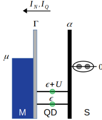
FIGURE 3.3. The system to be studied consists of a quantum dot (QD) with level \epsilon and Coulomb interaction U , weakly coupled to a normal metal (M) with coupling \Gamma and proximized by a superconductor (S) in the large gap limit with superconducting pairing strength \alpha . The black dots indicate a Cooper pair in the condensate. By convention the particle- and heat currents I_N and I_Q are directed into the normal metal.
