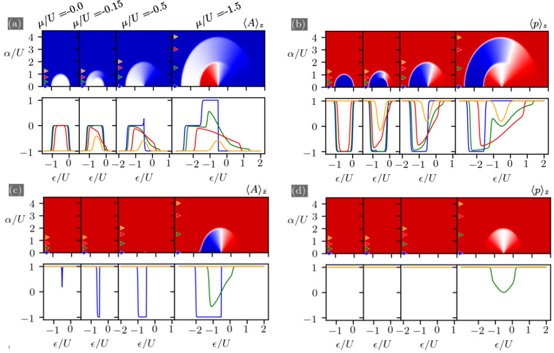
FIGURE 5.4. Expectation values of polarization A and parity p in the stationary state of the system (z) [(a) and (b)] and the dual system (\bar{z}) [(c) and (d)]. Parameters and conventions are the same as in Fig. 5.3.
