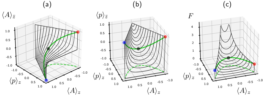
FIGURE 4.2. (a) Stationary polarization \langle A \rangle_{\bar{z}} and (b) parity \langle p \rangle_{\bar{z}} of the dual system as function of the stationary parity \langle p \rangle_z for various polarizations \langle A \rangle_z of the actual system [Eq. (4.54a)]. (c) Non-linear rescaling factor F as function of \langle A \rangle_z and \langle p \rangle_z [Eq. (4.54b)]. The self-duality condition F(\langle A \rangle_z, \langle p \rangle_z) = 1 (green 3D curve) holds along the curve \langle p \rangle_z = \langle A \rangle_z^2 (dashed green 2D curve) in the base plane, which includes the pure states |\pm\rangle (blue/red points) and the maximally mixed state (black point). The latter is the only state for which |\bar{z}\rangle = |z\rangle . Corresponding values are shown in (a) and (b).
