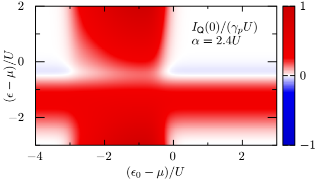
FIGURE 5.13. Initial total heat current after a slow switch at the chemical potential \mu = 1.2U and temperature T = 0.1U . The pairing is \alpha = 2.4U .
