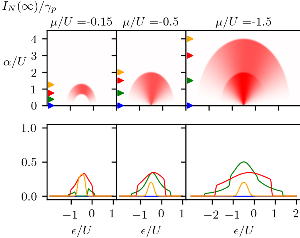
FIGURE 5.12. Stationary charge current I_N(\infty) with horizontal line cuts indicated by the corresponding arrows. Parameters and conventions are the same as in Fig. 5.3.
