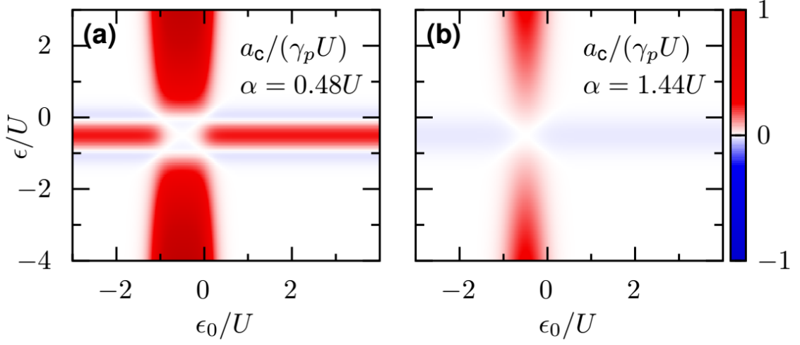
FIGURE 5.10. Heat current amplitudes after a slow switch at zero chemical potential and temperature T = 0.1U : (a) charge amplitude a_c for weak pairing \alpha = 0.48U and (b) a_c for strong pairing \alpha = 1.44U . The parity amplitude a_p is zero (not shown).
