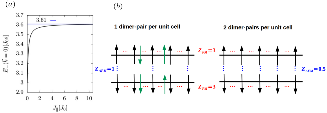
FIGURE 2.4. (a) Magnon gaps for a realistic (black line) and a hypothetical bilayer (blue line) as a function of the FM coupling strength J_{\parallel} . The anisotropy is constant with J_{\parallel}^{zz} - J_{\parallel} = 1.0 J_0 , J_{\perp}^{zz} - J_{\perp} = 0.3 J_0 and J_{\perp} = 1.0 J_0 . (b) Left: Realistic bilayer schematic with coordination numbers Z_{AFM} = 1 and Z_{FM} = 3 . Green arrows indicate deviations from the classical Néel state order. (b) Right: Hypothetical bilayer schematic with Z_{AFM} = 0.5 and Z_{FM} = 3 . For further explanation see the text.
