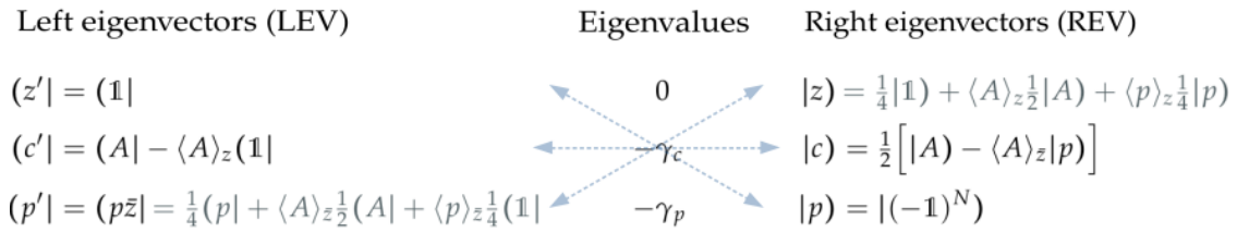
FIGURE 4.1. Left and right eigenvectors and eigenvalues of the kernel W . Their cross-relations are indicated by dashed arrows.
