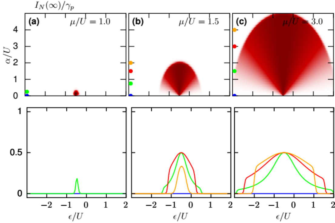
FIGURE 6.5. Stationary charge current I_N(\infty) for different values of the chemical potential and T = 0.02|U| . The upper plots show the current as function of the gate-voltage \epsilon = \delta - U/2 and induced pairing \alpha , while the corresponding bullets indicate the position of horizontal line cuts shown in the lower plots.
