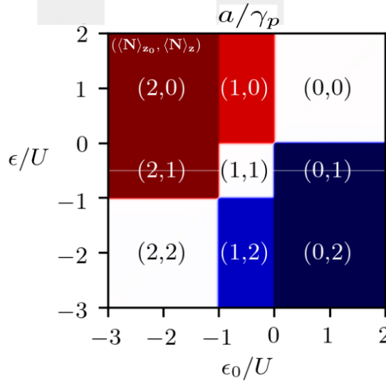
FIGURE 5.1. Gate-switch spectroscopy of a QD without superconductor ( \alpha = 0 ), attached to a normal metal (ND-device): Color-coded amplitude of the transient charge current [(a/\gamma_p)(\epsilon_0, \epsilon)] , Eq. (4.66), as a function of initial and final gate-voltages \epsilon_0, \epsilon before and after the switch, respectively. Dark/light-red (dark/light-blue) color indicates the current is directed into (out of) the metal. Possible integer charge values (\langle N \rangle_{z_0}, \langle N \rangle_z) in the initial and final stationary states z_0 and z before and after the switch, respectively, are indicated in the corresponding regions of the plot. For further explanation see the main text.
