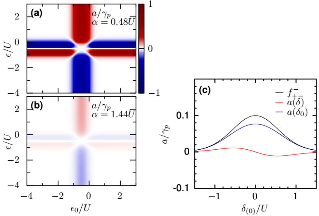
FIGURE 5.8. Charge amplitudes a after a slow switch at zero chemical potential and temperature T = 0.1U (a) for weak pairing \alpha = 0.48U and (b) for strong pairing \alpha = 1.44U . (c) For the final (initial) far off-resonant state |-\rangle = |0\rangle ( |-\rangle_0 ), a horizontal (vertical) linecut a(\delta_{(0)}) is given, respectively.
