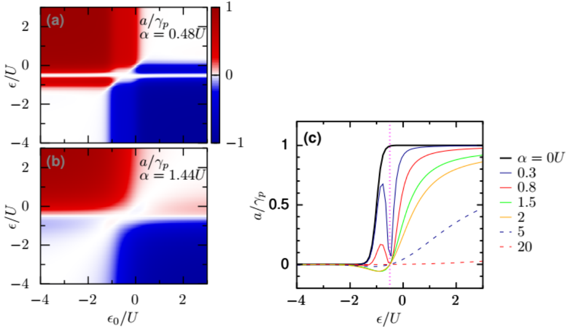
FIGURE 5.6. Charge amplitudes a after a fast switch at zero chemical potential and temperature T = 0.1U : (a) for weak pairing \alpha = 0.48U , (b) for strong pairing \alpha = 1.44U , (c) for different pairing strengths \alpha at initial gate voltage \epsilon_0 = -3U .
