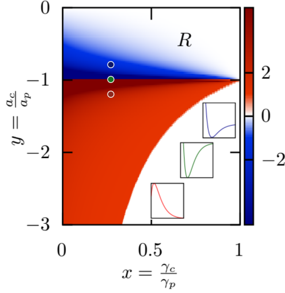
FIGURE 5.5. Possible values of the non-monotonicity quantifier R [Eq. (5.20)] as function of the possible values of the ratio of decay rates and of amplitudes. The insets show examples for non-monotonic profiles of the transient heat current as function of time for decay with a zero (blue, -1 \leq y < 0 ), for decay without a zero (red -1/x \leq y < -1 ) and an intermediate case (green, y = -1 ). In the latter case the transient heat current is both initially and finally zero.
