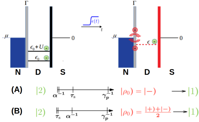
FIGURE 5.2. Schematics of an exemplary gate switch \epsilon(t) applied to a quantum dot (D) (center) when attached to a normal metal (N, dark blue) at chemical potential \mu and proximized with a superconductor (S, right) at potential zero. Black (red) bar indicates D is off (on) resonance with the proximity effect of S, respectively. Green bullets refer to the stationary charge of D before (top, left) and after the switch (top, right) with two types of possible particle transfers to the final state, as indicated by red arrows (top, right). (Bottom) Comparison of the different time scales \tau_s, \alpha^{-1}, \gamma_p^{-1} \equiv \Gamma^{-1} characterizing the two types of switches (A) slow and (B) fast as well as the resulting initial states |\rho_0\rangle . For further explanation, see the main text.
