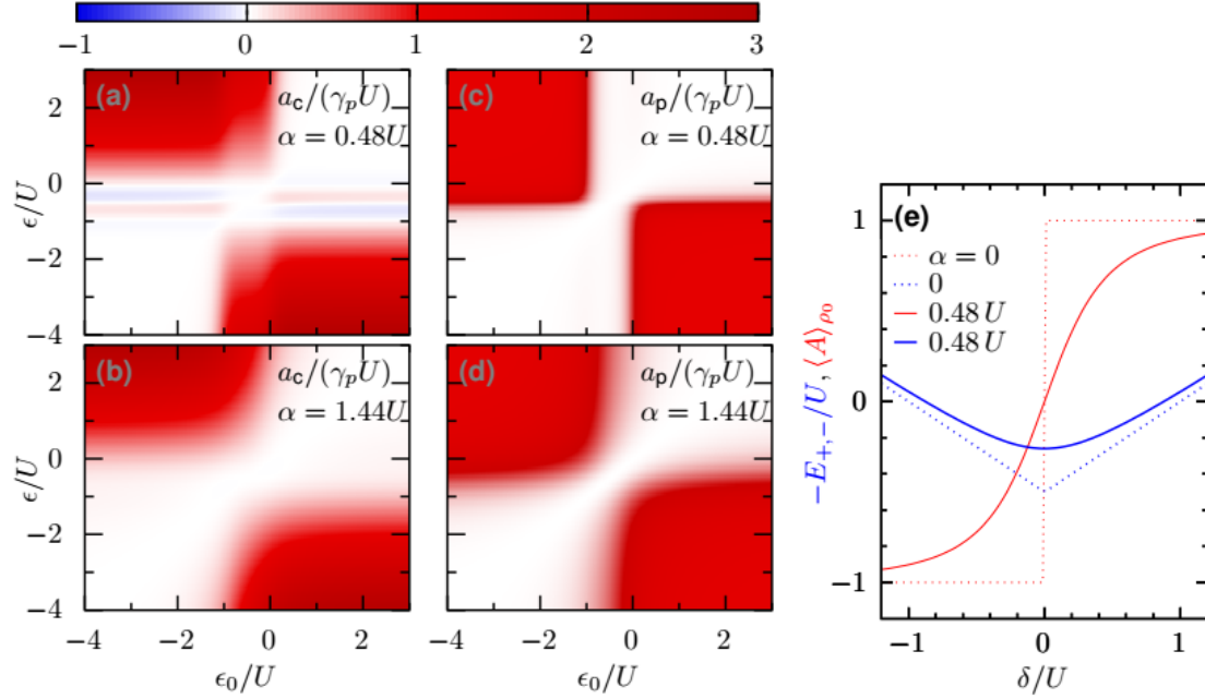
FIGURE 5.9. Heat current amplitudes after a fast switch at zero chemical potential and temperature T = 0.1U : (a) charge amplitude a_c for weak pairing \alpha = 0.48U and (b) a_c for strong pairing \alpha = 1.44U ; (c) parity amplitude a_p for weak pairing \alpha = 0.48U and (d) for strong pairing \alpha = 1.44U . (e) Heat current amplitude a_c decomposed into its factors, -E_{+-}/U (blue) and \langle A \rangle_{\rho_0} (red) for the case of weak pairing, \alpha = 0.48U (solid) and the normal conducting case \alpha = 0 (dashed). The initial state is off-resonant, |\rho_0\rangle = |2\rangle .
