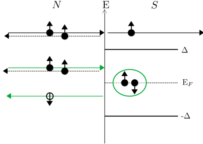
FIGURE 3.1. Possible transport processes at a normal metal-superconductor (NS) interface in dependence of energy E (vertical axis): An electron incident on the interface (black arrow) can be transmitted into the superconductor as a quasi particle (black arrow) only above the superconducting gap \Delta or it is back reflected as an electron into the normal metal (black dashed arrow). If incident below the gap (green arrow), it is either normally reflected (black dashed arrow) or Andreev reflected as a hole (green arrow), leaving in the latter case a Cooper pair in the superconductor.
