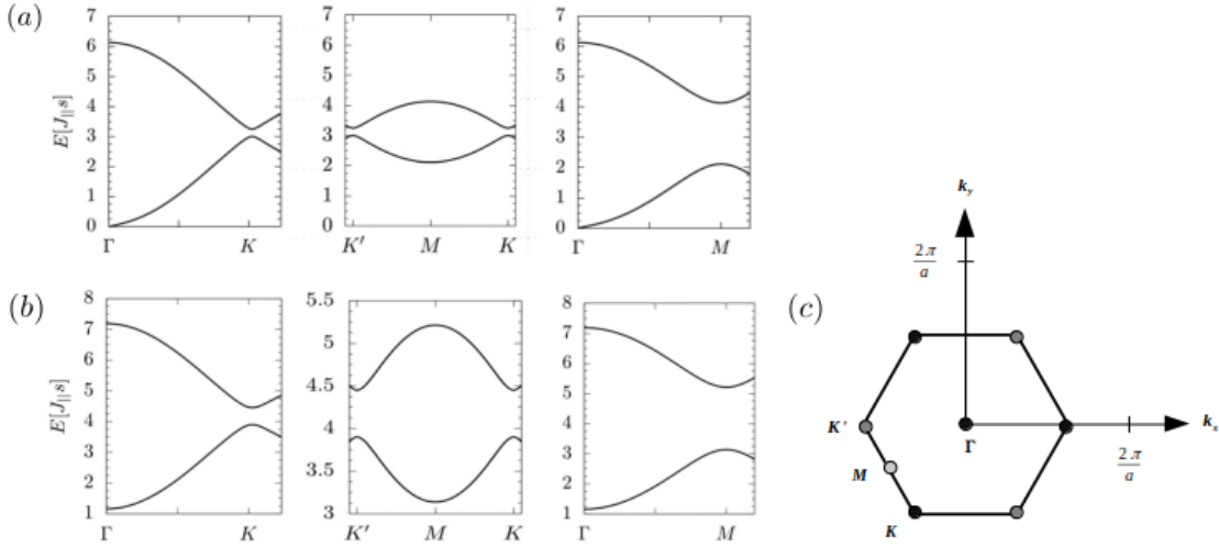
FIGURE 2.3. Dispersion of a bilayer with AFM inter-layer and FM intra-layer coupling. (a) For isotropic exchange coupling constants and a ratio of inter- vs. intralayer coupling J_{\perp} = 0.26 J_{\parallel} , (b) for anisotropic exchange coupling J^{zz} \neq J^{xx} = J^{yy} = J . Here the inter-layer couplings J_{\perp} = 0.26 J_{\parallel} , J_{\perp}^{zz} = 0.56 J_{\parallel} and intra-layer coupling J_{\parallel}^{zz} = 1.3 J_{\parallel} . (c) Wigner-Seitz cell of the reciprocal lattice with two types of equivalent Dirac-points K and K' and lattice points M, \Gamma .
