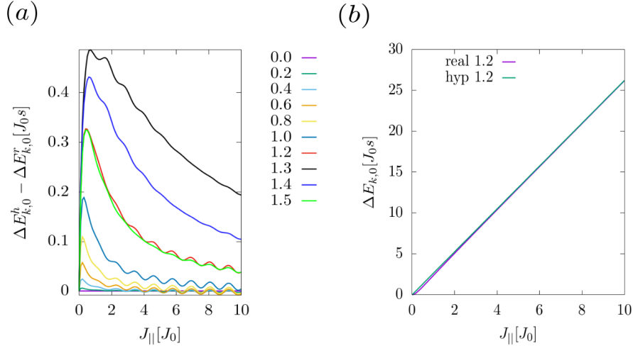
FIGURE 2.5. (a) Difference \Delta E_{k,0}^h - \Delta E_{k,0}^r between the hypothetical and the realistic bilayer structure as a function of the FM coupling for different values of (k_x, 0) in units of [\frac{\pi}{a}] along the \Gamma - K direction in the first BZ. (b) Energy difference \Delta E_{k,0} between a magnon with wavevector (1.2, 0)[\frac{\pi}{a}] and zero wavevector in the lower band as a function of the FM coupling strength J_{||} for bilayers I (green) and II (violet). For further explanation see the main text.
