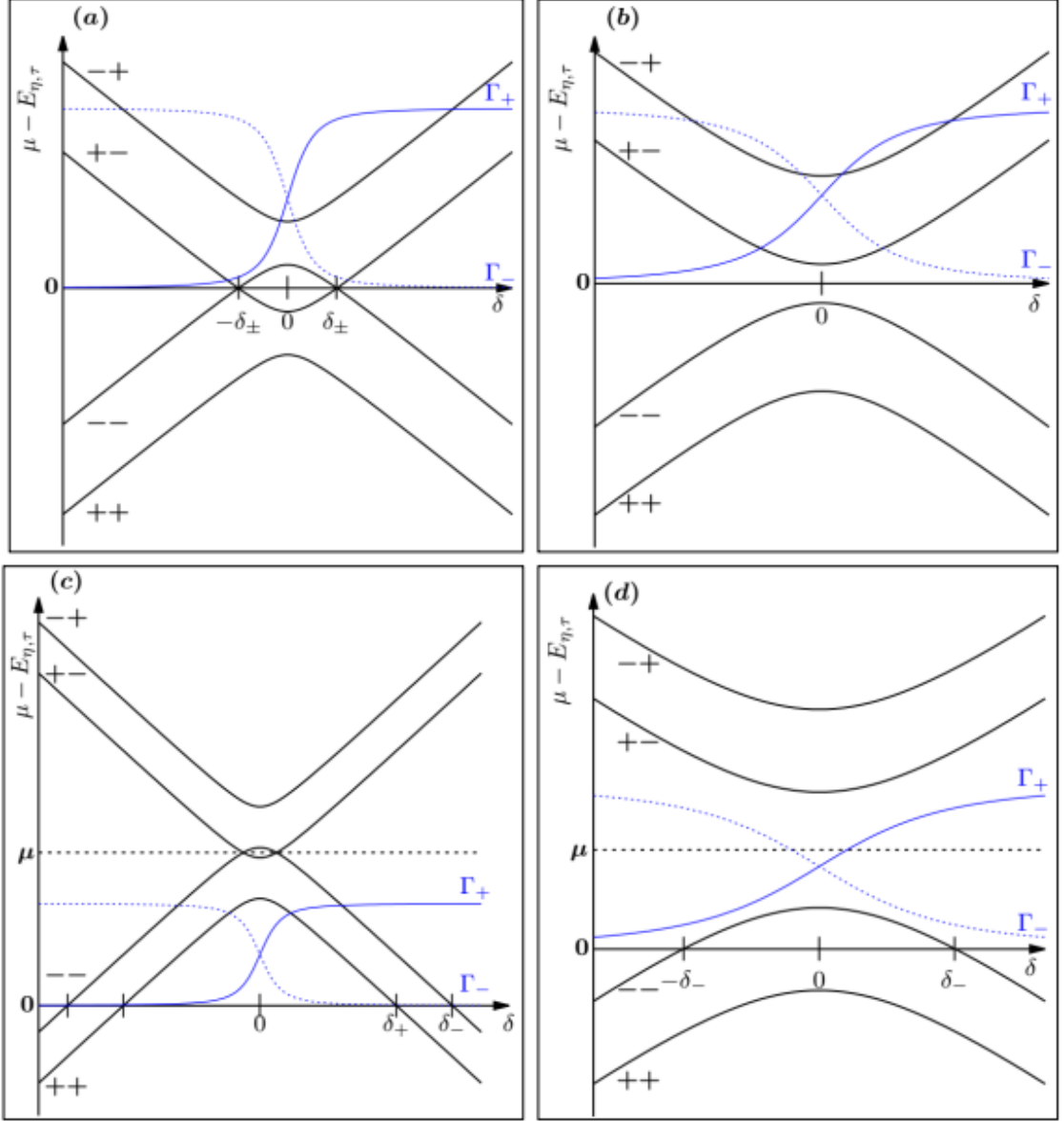
FIGURE 5.7. Schematic overview of zero temperature energy thresholds \mu - E_{\eta,\tau} (Table 3.1) for the cases of (a) \mu = 0 and weak pairing \alpha , (b) strong \alpha , (c) \mu > 0 and weak \alpha and (d) moderate \alpha . \delta_{\pm} specifies the region of detuning, as introduced in Sec. 5.2.1.
