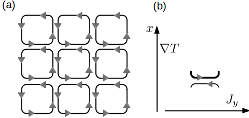
FIGURE 2.6. Magnon Hall effect schematically, drawn after [29]. A transverse magnon Hall current J_y develops in response to a longitudinal temperature gradient \nabla T \parallel \hat{x} , the x -direction as indicated in (b). (a) The 2D sample is constructed from small neighboring confined regions, shown are the edge currents. (b) In the presence of a temperature gradient, edge currents of neighboring regions J_y(x) \neq -J_y(x + \Delta x) no longer cancel out and therefore result in a net transversal current (magnon Hall current).
