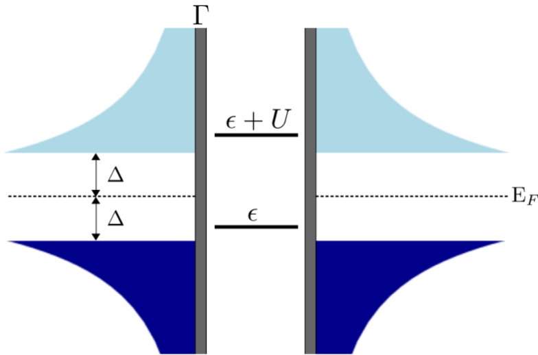
FIGURE 3.2. A quantum dot attached to superconducting reservoirs (SDS-device) schematically: Indicated are the single level QD with energy level \epsilon , charging energy E_C = U/2 and tunnel coupling strength \Gamma to the two superconductors. Their BCS-density of states is indicated in blue with the superconducting gap \Delta . The states are here filled (dark blue) up to the Fermi energy E_F .
