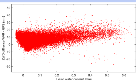
Figure 4. ZWD differences: WVR–GPS.
