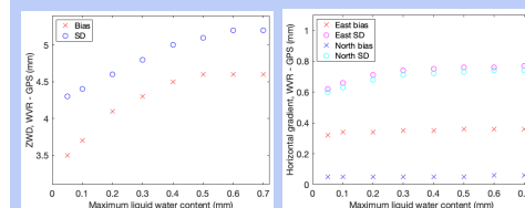
Figure 5. The bias and SD for WVR–GPS differences of the ZWD (left) and the horizontal gradients (right). The number of data points is reduced from 77,966 for \text{LWC} < 0.7 mm to 56,176 for \text{LWC} < 0.05 mm.
