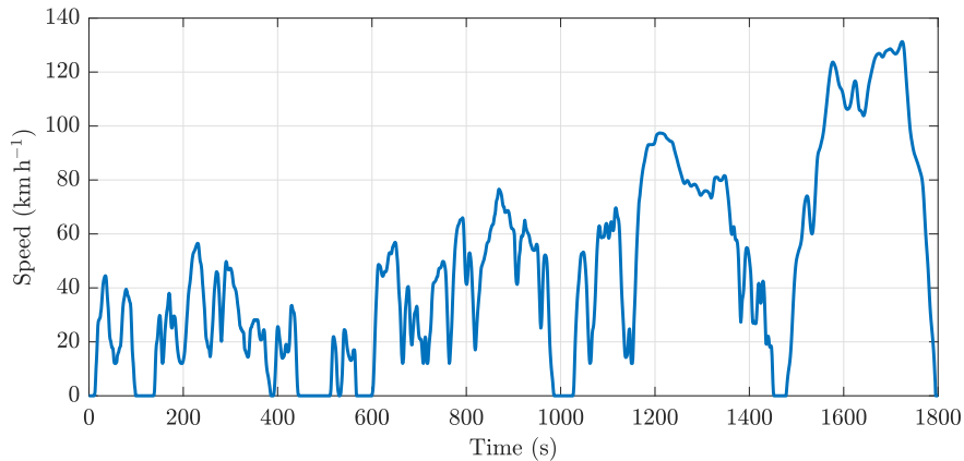
Figure 1.2: The WLTC class 3 driving cycle.
