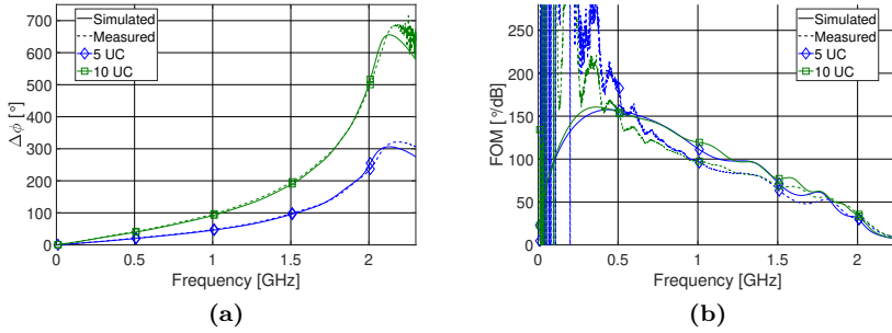
Figure 4.11. (a) The differential phase shift between V_{Rmin} = 3 V and V_{Rmax} = 8 V for and (b) FOM for phase shifters with a unit cell length of 66.4^\circ .
