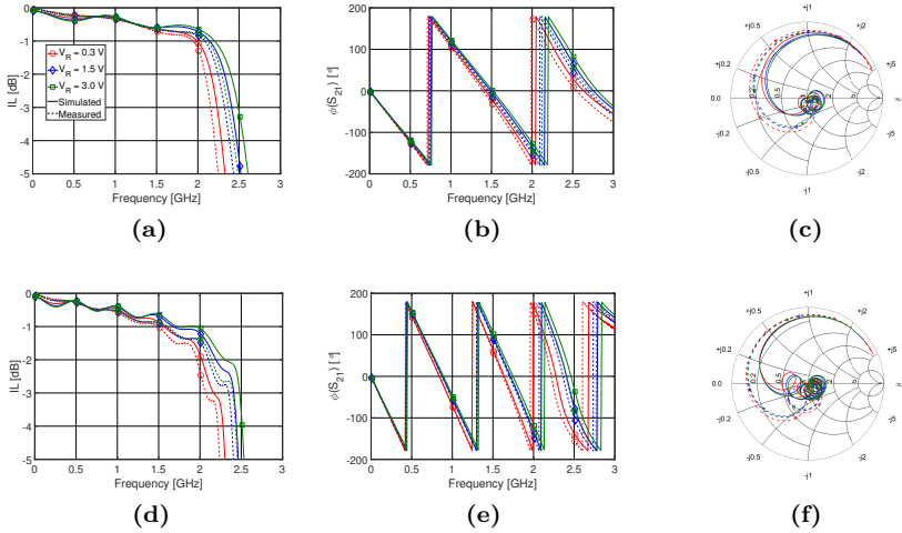
Figure 4.8. The simulated and measured S-parameters for the phase shifter in Paper B. The results for the phase shifter with 4 unit cells (a) IL , (b) phase shift, and (c) |S_{11}| . The results for the phase shifter with 7 unit cells (d) IL , (e) phase shift, and (f) |S_{11}| .
