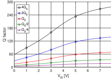
Figure 5.6. The quality factor at 1.5 GHz for the varactor-diodes employed in the phase shifters compared.
