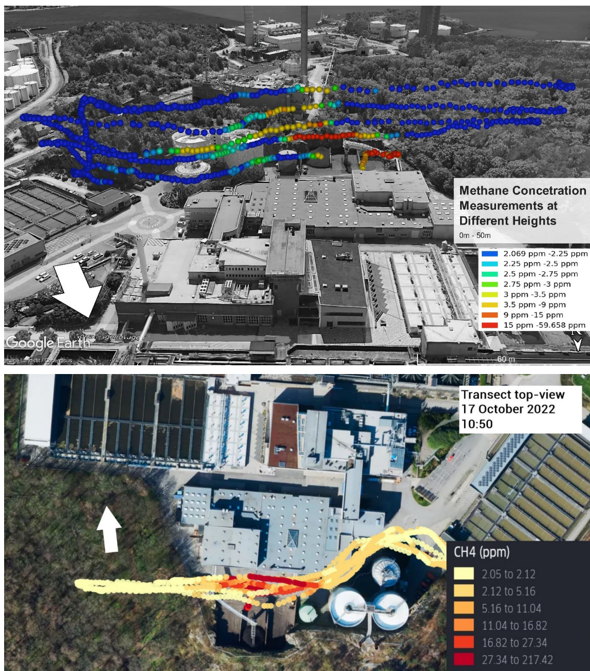
Figure 20. A typical example of a "wall transect" downwind of the sludge piles at the WWTP plant on October 17, 2022. These transects were carried out at various heights, from 0m to 50m. The spheres indicate methane measurement points, and each colour indicates absolute concentration in ppm above background level. White arrow indicates wind direction. Map: Google Earth™ © 2022.. The lower graph visualizes the flight path of the drone as seen from above. Graphic from: www.kepler.gl with underlying Map from Mapbox©.
