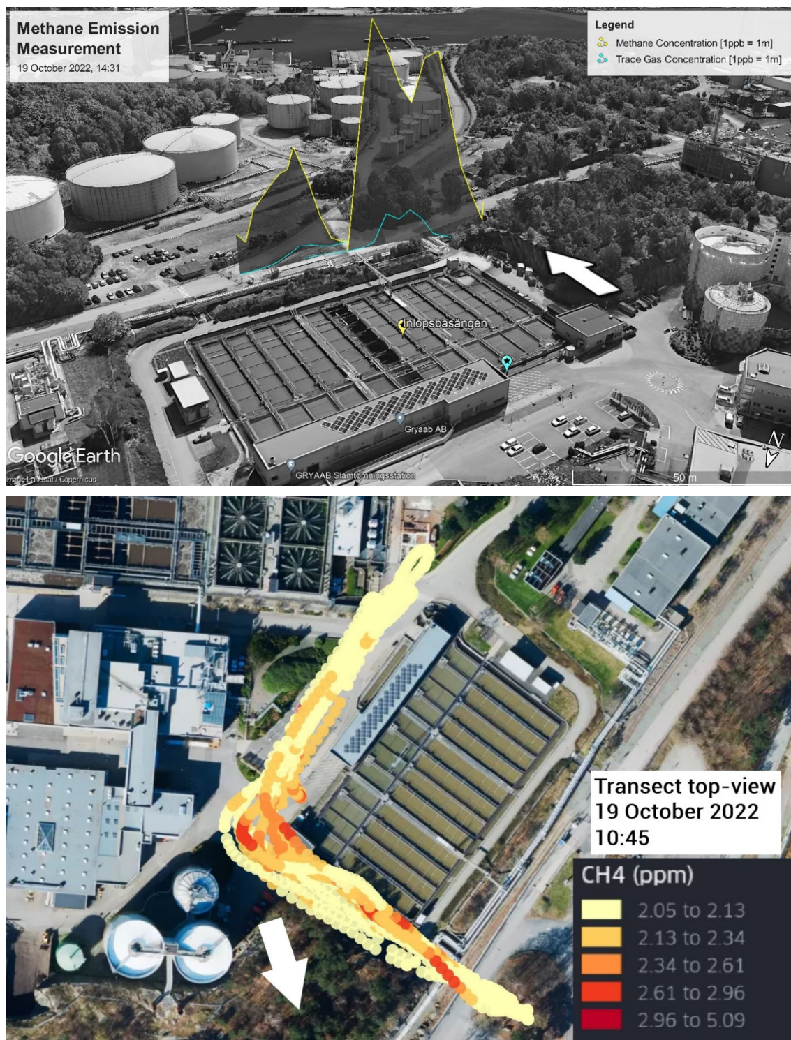
Figure 17. Example of a drone-based methane measurement at the primary clarifiers of the WWT plant on October 19, 2022, carried out at 14:31. In the upper graph The height of the curves corresponds to the concentration of the measured gas at ground level (above background concentration). The highest measured methane concentration at this measurement was 301 \mu\text{g}/\text{m}^3 . See Figure 3 for a general description of the graph structure. Map: Google Earth™ © 2022. The lower graph visualizes the flight path of the drone as seen from above. Graphic from: www.kepler.gl © with underlying Map from Mapbox©.
