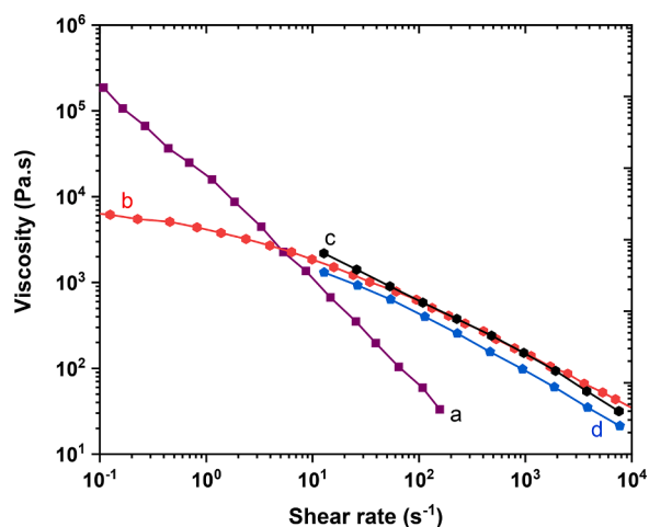
Fig. 8. Viscosity – shear rate relationships of (a) acetylated lignocellulose pulp at 120 \text{ }^\circ\text{C} (b) LDPE at 150 \text{ }^\circ\text{C} , (c) WPC (wood/polypropylene ratio: 40/60) at 180 \text{ }^\circ\text{C} and (d) WPC (wood/polypropylene ratio: 20/80) at 180 \text{ }^\circ\text{C} (Wilczyński & Buziak, 2021). The viscosity of acetylated lignocellulose was measured using rotational rheometer while capillary rheometer for LDPE and WPC. Redrawn from: (a) Li et al., 2021b, (b) Zatloukal, 2016, (c) and (d) (Wilczyński & Buziak, 2021).
