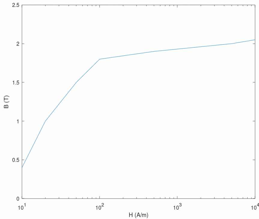
Figure 21. BH-curve of the grain-oriented material.
