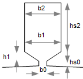
Figure A1. Slot dimensions
