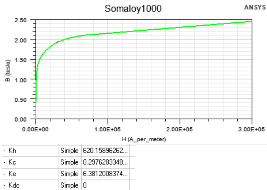
Figure 2. Soft magnetic material
