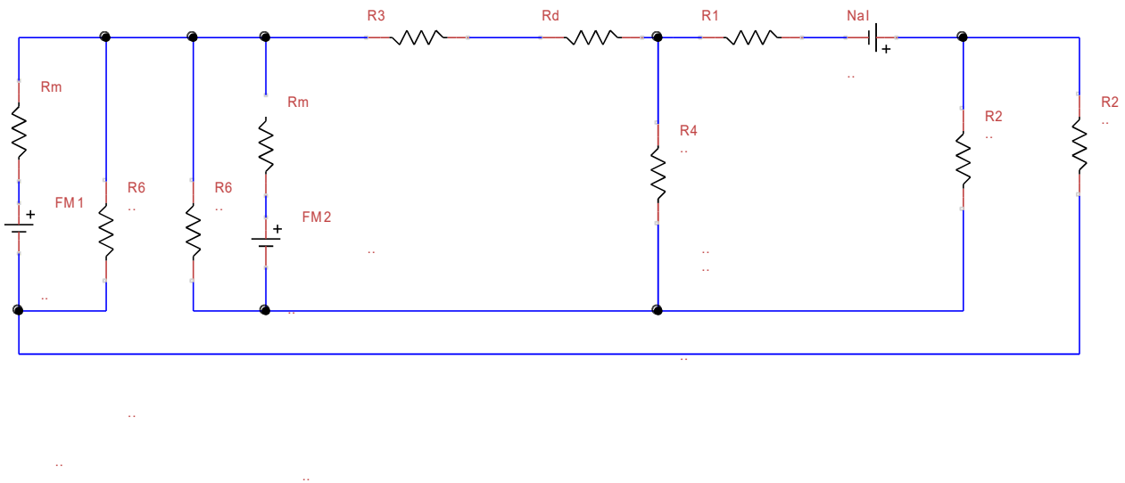
Figure. 6 Reluctance model of pole.
