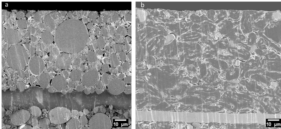
Figure 3.1: SEM of cross section of (a) positive NCA electrode and (b) negative \text{SiO}_x electrode. The metallic current collectors visible in lower part of images, the active material particles of various sizes and shapes above. Reproduced from Paper III under CC BY NC ND 4.0 license.
