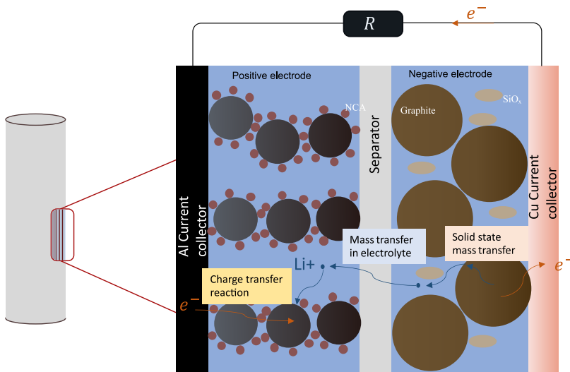
Figure 2.2: Graphic summary of physical processes in battery during discharge and their connection to the DFN model. \text{Li}^+ ions are released from the negative electrode, in pairs with electrons, in a charge transfer reaction. They are then separated and electrons transported through external circuit while \text{Li}^+ transport happens through the liquid electrolyte as mass transfer. \text{Li}^+ and electrons then combine in charge transfer reaction on positive electrode surface and diffuse to a free site in the porous electrode via solid state mass transfer.
