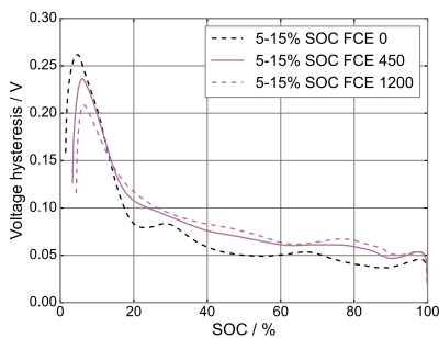
Figure 4.7: Comparison of the voltage difference between the charge and discharge part at the same SOC during C/20 cycling for (a) a full cell at BOL, (b) a cell cycled in 5-15% SOC window at three ageing stages, and (c) a cell cycled in 85-95% SOC window at different stages of ageing. Reproduced and adapted from Paper II .
