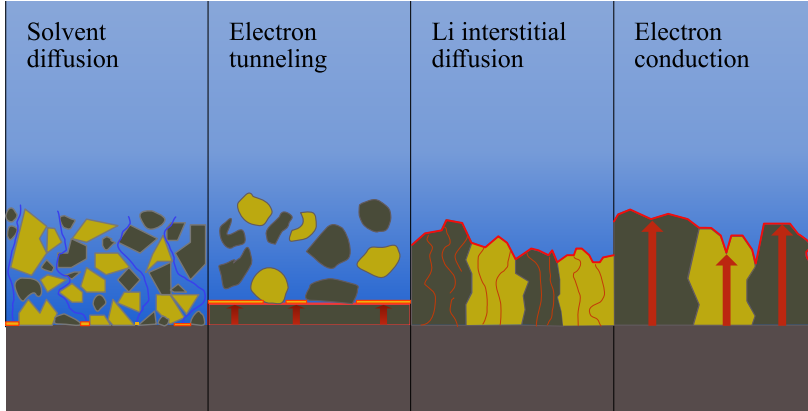
Figure 2.3: Schematic illustration of the four suggested growth models detailed in Section 2.3.1. Red and orange indicate regions where SEI growth is happening, arrows and curves indicate transport of species involved in reaction
