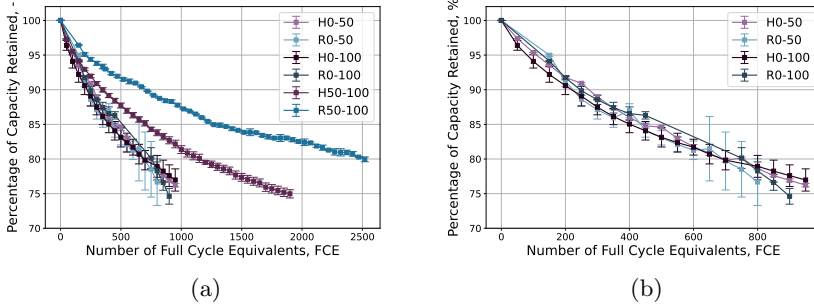
Figure 4.3: Capacity fade cells tested in large SOC windows. All cells shown in (a) with a subset of cells cycled to 0% SOC shown in (b) to improve visibility. Legends are consistent with test tag in Table 3.2. Reproduced from Paper III .
