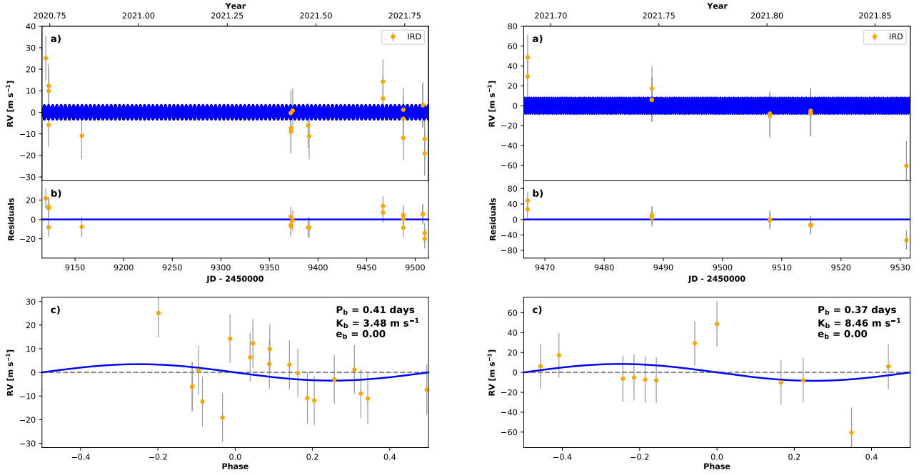
Fig. 7. Radial velocity data and maximum likelihood radvel1 models for TOI-1442 (left) and TOI-2445 (right). The top panels display the full timeline data, while the bottom panels show the phase-folded data using the best-fit orbital parameters. The error bars do not account for systematic offsets.
