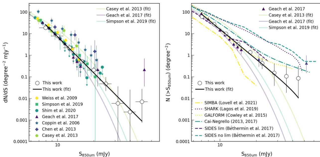
Figure 14. Number counts of 850 \mu\text{m} sources measured from the S2LXS XMM -LSS survey 5\sigma catalogue (white circles with black outline). In the left-hand panel, we present the differential number counts from this work along with observational constraints from S2CLS (Geach et al. 2017), S2COSMOS (Simpson et al. 2019), and the other main blank-field surveys (Coppin et al. 2006; Weiß et al. 2009; Casey et al. 2013; Shim et al. 2020), as well as from Chen et al. (2013) who combine data from two cluster lensing fields and three blank fields. The S2LXS XMM -LSS differential number counts are consistent with these previous studies within the uncertainties for the flux range probed. We find an excess in the number counts [above the Schechter (1976) function fit of Geach et al. (2017)] at \gtrsim 15 mJy, similar to that found in S2CLS (Geach et al. 2017). In the right-hand panel, we present the S2LXS XMM -LSS cumulative number counts, comparing both to observations and several simulated galaxy models. For clarity, we only plot the observational constraints from S2LXS XMM -LSS and S2CLS, and the model fits from S2COSMOS and Casey et al. (2013). We show the 850 \mu\text{m} number counts from semi-analytical models (Cowley et al. 2015; Lagos et al. 2019), empirical models (Cai et al. 2013; Béthermin et al. 2017; Negrello et al. 2017) and the cosmological hydrodynamical simulation SIMBA (Lovell et al. 2021). The results from Lovell et al. (2021) and Cowley et al. (2015) both take into account blending from a 15-arcsec beam. The Béthermin et al. (2017) standard model has a star formation rate limit of 1000 M_{\odot} \text{yr}^{-1} . We show the results both with and without this limit. The Béthermin et al. (2017) models shown do not take account of blending, but do include a prescription for lensing. The Cai–Negrello model combines the counts of unlensed and strongly lensed galaxies. The excess in the S2LXS XMM -LSS number counts at \gtrsim 15 mJy is most consistent with the results from the Cai–Negrello empirical model (Cai et al. 2013; Negrello et al. 2017), the semi-analytical model of Cowley et al. (2015), and the standard empirical model of Béthermin et al. (2017). The error bars in both panels show Poisson uncertainties (Gehrels 1986).
