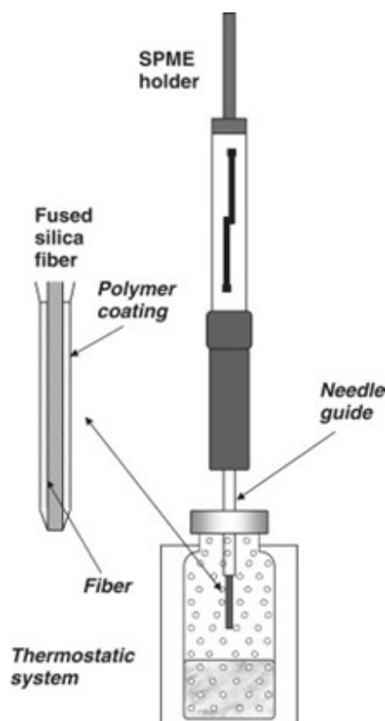
Figure 4.4: SPME for volatile compounds collection [125].
