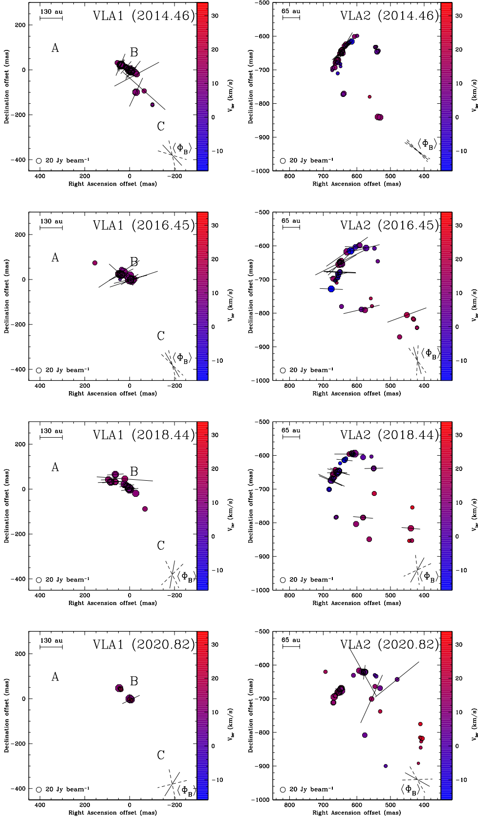
Fig. A.1. Close-up view of the 22 GHz H 2 O maser features detected around the radio sources VLA 1 (left panels) and VLA 2 (right panels) in epochs 2014.46 (top panels), 2016.45, 2018.44, and 2020.82 (bottom panels). The reference positions are reported in Table 2. The letters A, B, and C indicate the position of the three maser groups identified around VLA 1 by S11a and they are reported here only for reference. The octagonal symbols are the identified maser features scaled logarithmically according to their peak intensity (Tables A.1-A.8). Maser LSR radial velocities are indicated by color (the assumed systemic velocity of the region is V_{\text{lsr}} = +10.0 \text{ km s}^{-1} ; Shepherd et al. 2003). The linear polarization vectors, scaled logarithmically according to the polarization fraction P_1 , are overplotted. In the bottom-right corner of all panels the error-weighted orientation of the magnetic field ( \langle\Phi_B\rangle ) is also reported; the two dashed segments indicate the uncertainties.
