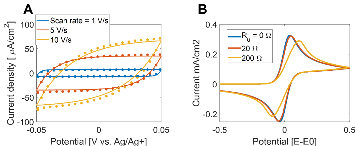
Figure 13 A) Fast CV sweeps on an ITO electrode exhibit a capacitive behavior (dotted) where a simulation of an RC-circuit (solid) fits perfectly with the parameters R = 200 \Omega and C = 7 \mu\text{F} . B) How the uncompensated resistance affects the CV. Peak separation is visible with higher uncompensated resistance.
