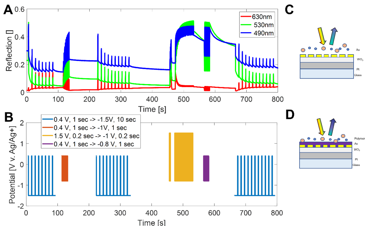
Figure 42 A) Reflection trace of three wavelengths representing red (630 nm), green (530 nm) and blue (490 nm) colors. B) The applied potentials waveform. C) A schematic of the cavity with WO 3 as a spacer layer. D) A schematic of the cavity with the polymer PProDOT-Me 2 on top of the gold.
