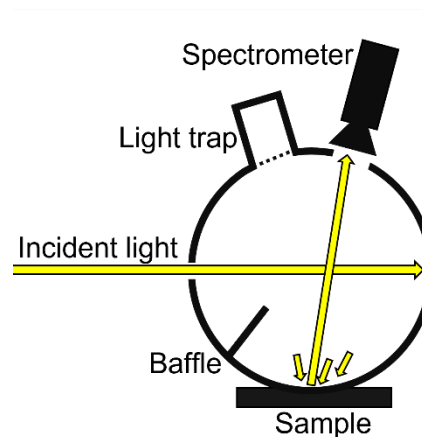
Figure 29 Light is illuminating the integrated sphere which produces diffuse light. The sample is illuminated with diffuse light and the reflection is measured.
