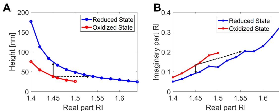
Figure 41 The fitted height against the n -value for both oxidized and reduced. B) The fitted k -value for each n -value for both reduced and oxidized. The arrows indicate two different scenarios upon reduction. The wavelength is 785 nm.
