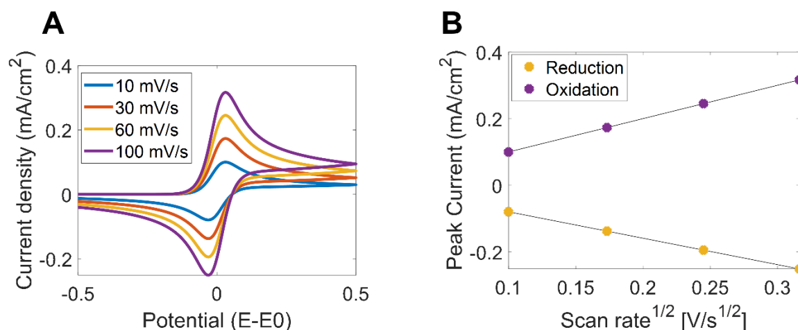
Figure 9 A) Simulations of CV diagrams for various scan rates. The concentration is 1 mM and the diffusion constant is 1.5 \times 10^{-5} \text{ cm}^2/\text{s} . B) The peak currents plotted against the square root of the scan rate displays a linear relationship.
