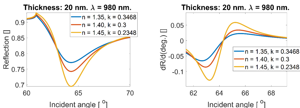
Figure 39 The minimum in the angular spectra depends on both the n -value and the k -value. The width of the dip is determined by the k -value. In the differentiated spectra the slope around the minimum is then determined by the k -value.
