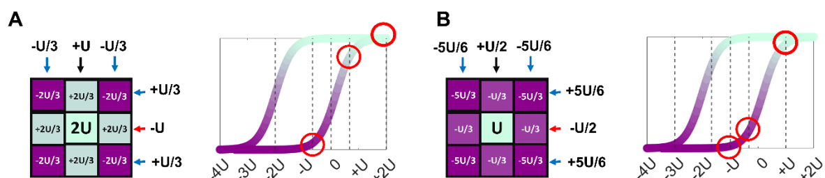
Figure 24 The middle pixel is being addressed. A) If the EO curve is not centered around the zero (0) but shifted crosstalk will still be present. B) By adjusting the potentials the crosstalk voltages can be shifted as well.
