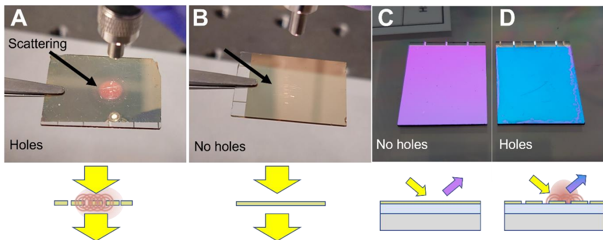
Figure 7 A) White light impinging on a gold surface with nanoholes exhibit red scattering. B) Planar gold does not exhibit this. C) In a structural color pixel this can enhance coloration by D) scatter away red light.
