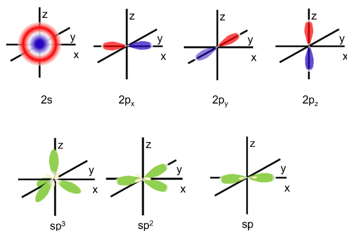
Figure 14 Top row: Orbitals of the valence electrons of carbon from the symmetric 2s to the three variations of the 2p-orbitals. The different shading of the 2p-orbitals represents the sign of the orbitals wavefunction. The bottom row: The three different hybridizations going from sp^3 to sp^2 and finally sp .
