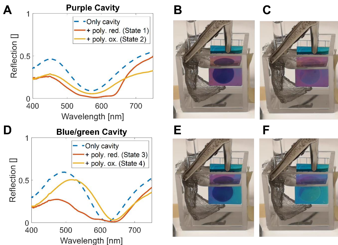
Figure 43 A) Spectra of only the cavity in purple state (--) and the cavity in purple state with PProDOT-Me 2 on top in either its colored or bleached state (-). B) A photo of State 1 and C) State 2. D) Spectra of only the cavity in blue/green state (--) and the cavity in blue/green state with PProDOT-Me 2 on top in either its colored or bleached state (-). E) A photo of State 3 and F) State 4.
