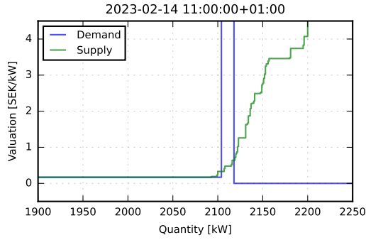
Figure 4.8: Supply and demand curves at hour 11 on the 14th of Feb. for case LFM+PT+ET
