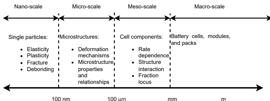
Figure 3.2: Mechanical properties of lithium-ion batteries at different length scales [74].
