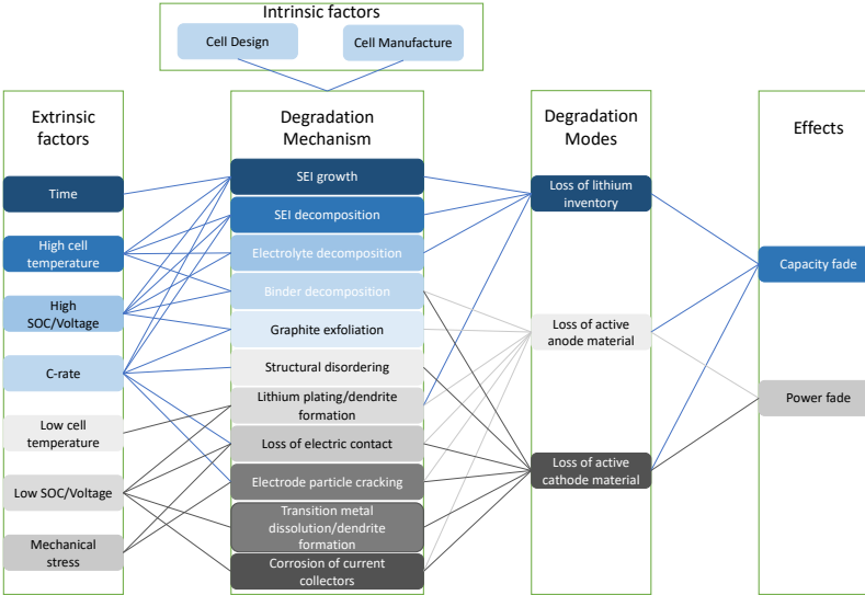
Figure 2.3: Cause and effect of dominant degradation mechanisms and their associated degradation modes [3] [55] [43].
