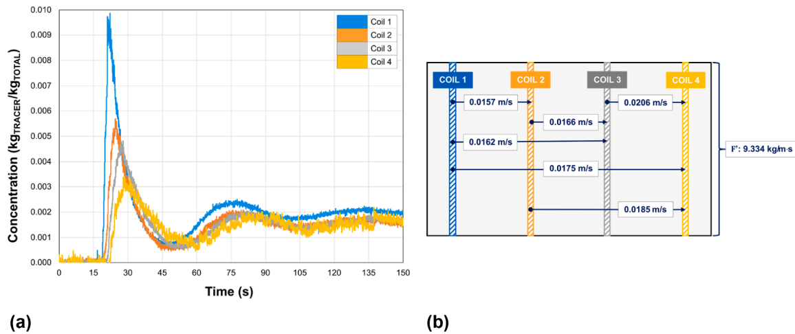
Fig. 9. Example of an analysis based on the magnetic solids tracing technique. Experimental conditions are set at: FN, 1.83; bed height, 100 mm; and volumetric flow rate in the conveying zone, 855 l_h/min . (a) Transient concentration profile. (b) Derived solids velocity values.
