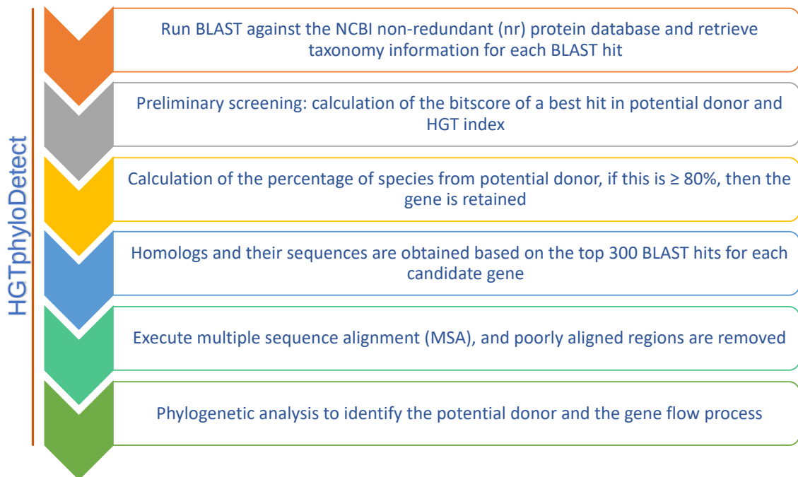
Figure 19 HGTphylloDetect workflow for automated detection of HGT events from closely related organisms (e.g., eukaryote-to-eukaryote transfers).
