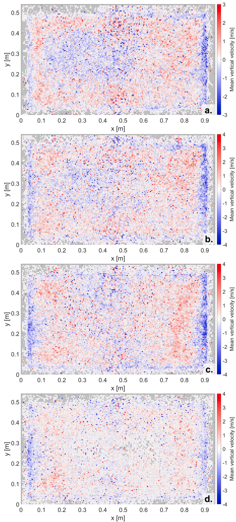
Fig. 6. Vertical tracer velocity over the horizontal plane, for a bed height of 130 mm and using a tracer particle with diameter of 18 mm and density of 1,015 kg/m 3 . Fluidization velocities used: a) 0.2 m/s; b) 0.3 m/s; c) 0.4 m/s; d) 0.5 m/s.
