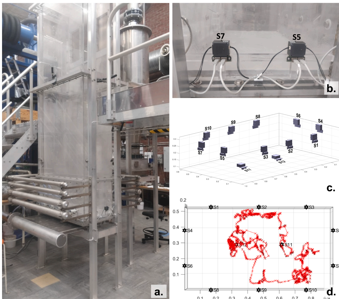
Fig. 1. A. Cold flow model of a circulating fluidized bed boiler. Cross-sectional area, 0.45 \text{ m}^2 ; total height, 3.1 m. B. Image of two of the sensors used for Magnetic Particle Tracking, positioned on the lateral walls of the cold model. C. Isometric schematic showing the allocation of the 12 sensors, 10 of which are positioned vertically on the lateral walls, while 2 are positioned horizontally underneath the cold model. D. Example of the trajectory of a tracer, acquired during 60 s; top view of the trajectory, indicating for each position the direction of the magnet polarization.
