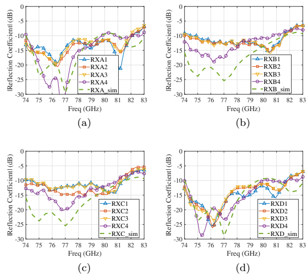
FIGURE 23. Reflection coefficients of RX slot arrays.
