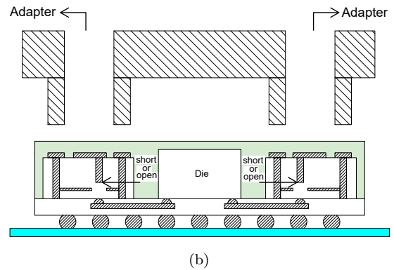
FIGURE 18. Testing structure for the interconnect and launcher: (a) configuration of RXs and TXs; (b) sectional view.
