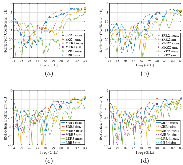
FIGURE 24. Reflection coefficients of TX slot arrays.
