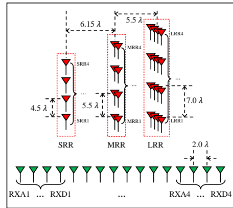
FIGURE 9. Antenna system of the simultaneous multi-mode automotive IMR with 12 Tx and 16 Rx [9].
