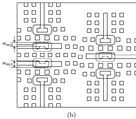
FIGURE 7. Compact transitions from the interconnects to the distribution layer: (a) 3D view, (b) top view.
