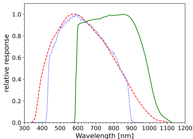
Fig. 1. Wavelength-dependent response functions of CHEOPS (dashed red), Kepler (dotted blue), and TESS (solid green). The response functions are from the Spanish Virtual Observatory Filter Profile Service (Rodrigo et al. 2012; Rodrigo & Solano 2020).
