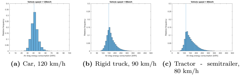
Figure 3.6: Air drag energy consumption distributions for driving with constant speed between Malmö - Göteborg from 2000-01-01 to 2022-03-01
