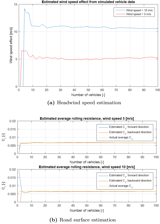
Figure 3.1: Road weather estimation from multiple vehicles
