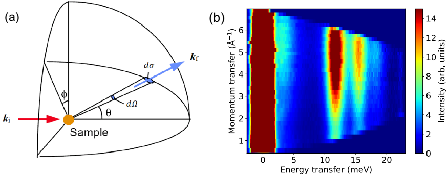
Figure 4.1: (a) Illustration of the scattering geometry in a neutron scattering experiment in real space. Adapted from [169, 172]. (b) INS data of a powder sample of \text{MAPbI}_3 at 2 K. The data were measured on the IN5 spectrometer at the Institut Laue-Langevin using an incident neutron wavelength of 1.7 \text{ \AA} .
