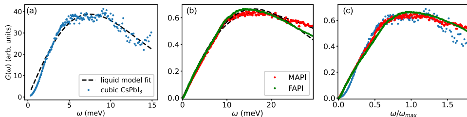
Figure 6.12: GDOS of (a) CsPbI 3 and (b) MAPbI 3 and FAPbI 3 in their high-temperature cubic phases. The data for CsPbI 3 is obtained at 600 K, and the data for MAPbI 3 and FAPbI 3 is taken at 350 K. The GDOS is fitted to the liquid vDOS model of Eq. (6.2) (black dashed lines). (c) Comparison of the GDOS of cubic CsPbI 3 , MAPbI 3 , and FAPbI 3 plotted on a scaled energy axis \omega/\omega_{\max} , where \omega_{\max} is the energy in which the GDOS shows a maximum.
