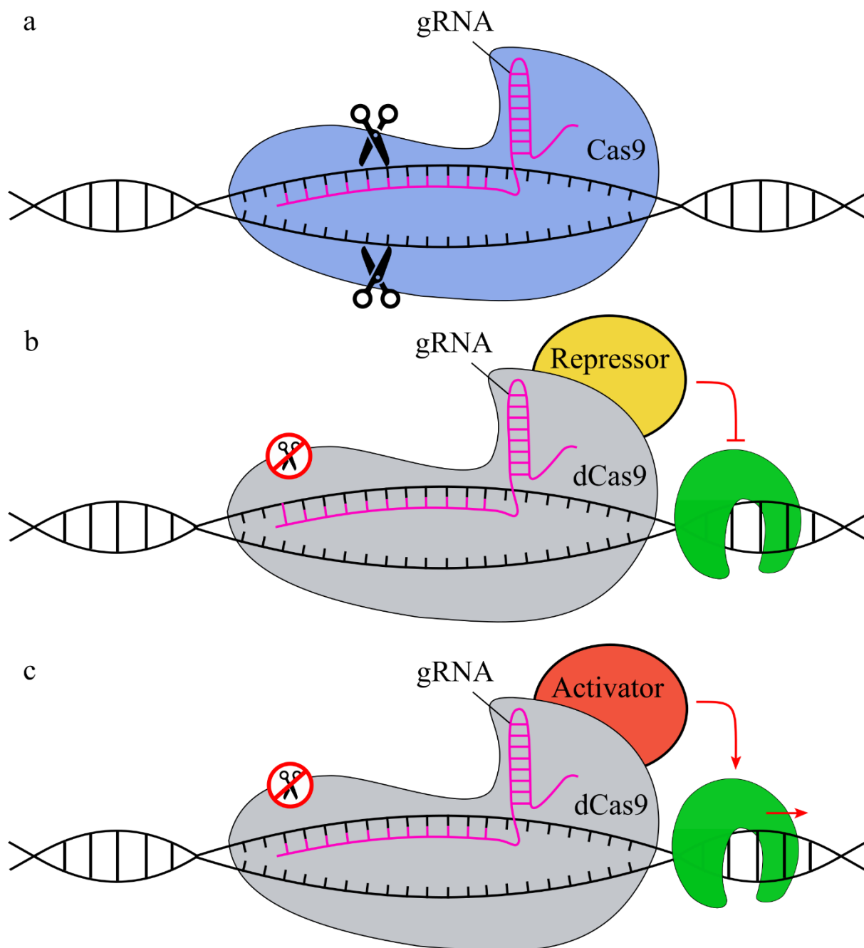
Figure 2.2: Schematic representation of CRISPR/Cas9 technologies. a) Classic CRISPR/Cas9, with gRNA driving the Cas9 endonuclease to the target sequence, where it can cleave the DNA. b) CRISPRi and c) CRISPRa mechanisms for gene repression or induction, respectively. Cas9 is deprived of its endonuclease activity (dCas9) and fused to a repressor/activator to prevent or facilitate the recruitment of the transcription machinery (here represented in green) and expression of the target gene.
