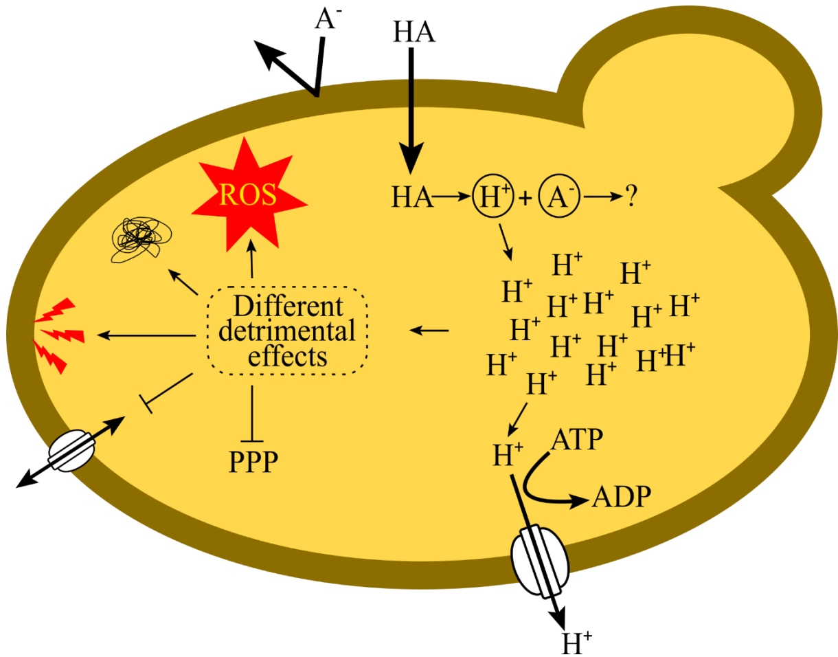
Figure 4.1: Inhibitory mechanism of acetic and formic acids. In their undissociated form (HA), acetic acid and formic acid can freely enter the cell and, once in the cytosol, they dissociate into protons ( H^+ ) and anions ( A^- ). While any toxic effect of the anionic form remains unclear, intracellular proton accumulation triggers the activity of ATP-dependent proton pumps, which maintain the physiological pH in the cytosol. The intracellular accumulation of protons causes different cytotoxic effects, including acidification of the cytosol, ATP depletion, ROS accumulation, protein aggregation, disruption of the cell membranes, inhibition of membrane trafficking, and inhibition of the pentose phosphate pathway (PPP).
