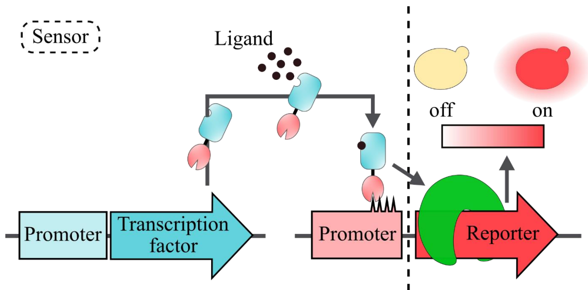
Figure 3.4: Schematic representation of a transcription factor-based biosensor mechanism. A transcription factor capable of recognizing the target molecule is expressed in the host. Upon binding to the target ligand, the transcription factor recognizes the binding sites in the reporter's promoter and recruits the transcription machinery (here represented in green) to express the reporter. The magnitude of the output signal generated by the reporter depends on how many transcription factor units bind the promoter. The sensor part of the biosensor, including the transcription factor and the promoter driving the expression of the reporter, is displayed on the left of the dashed line. On the right, the reporter gene is shown.
