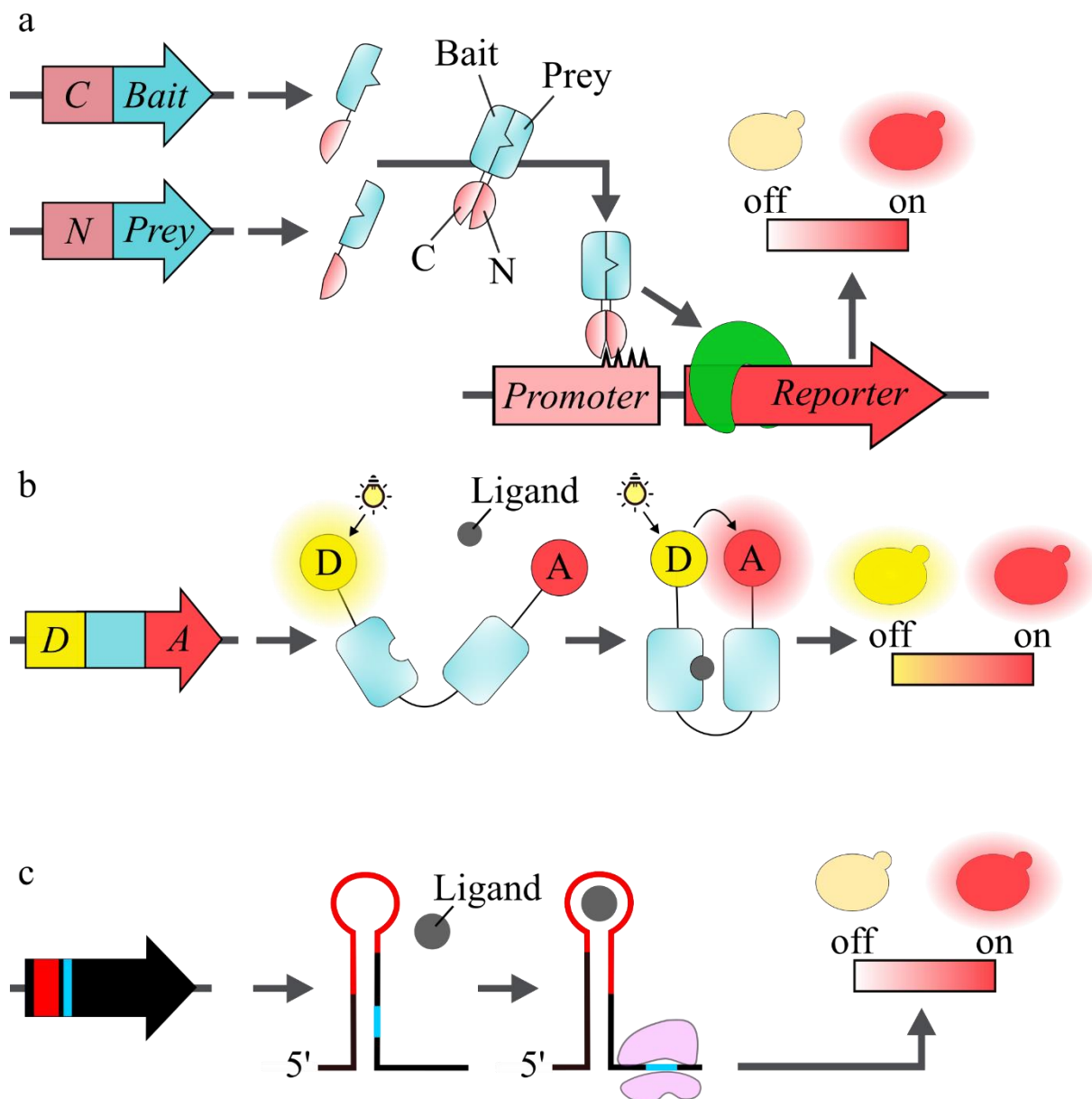
Figure 3.3: Schematic of different types of genetically encoded biosensors. a) Example of two-hybrid system biosensor where the bait protein and the prey protein are fused to the C-terminal domain (C) or the N-terminal domain (N) of Gal4. If prey and bait interact, Gal4 functionality is restored and it can recruit the transcription machinery (here in green) activating the reporter expression. b) Example of FRET-based biosensor where donor (D) and acceptor (A) are expressed in the same protein. Upon binding to the target molecule, the protein changes its conformation, approaching the light-excited donor to the acceptor. The acceptor gets excited by the donor generating a fluorescence emission. c) Example of RNA-based biosensor where the aptamer riboswitch (here the red lines), upon binding to the target molecule, induces a conformational change of the mRNA structure. The conformational change allows the ribosome (here in pink) to recognize the ribosome binding site (here the cyan lines) and start the translation of the reporter.
