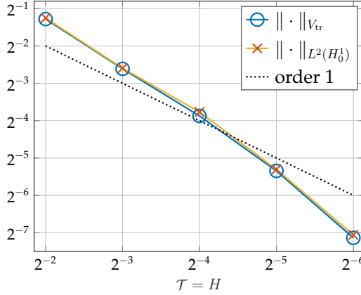
Figure 4.7: Relative error with respect to different space-time grid sizes H = T .
