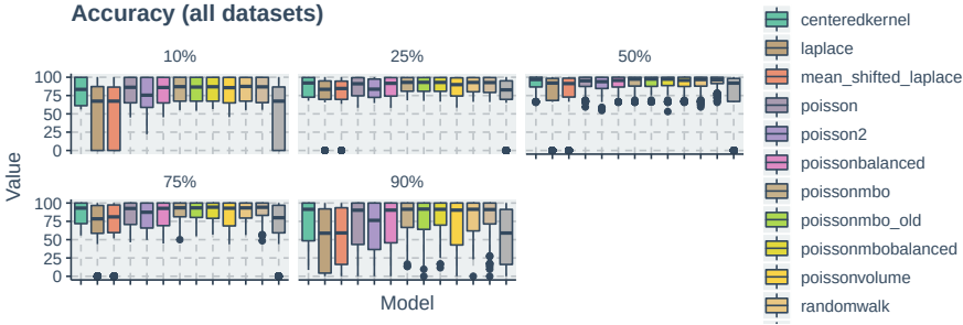
Figure 7.3: Boxplots illustrating the accuracy of all algorithms. From left to right in the upper row, we have boxplots for 10%, 25% and 50%. From left to right in the lower row, we have 75% and 90% available labels
