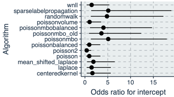
(g) HPDIs of the ORs for each algorithm intercept for 75% available labels.
