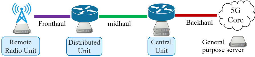
Figure 2.6: RAN architecture [10].
