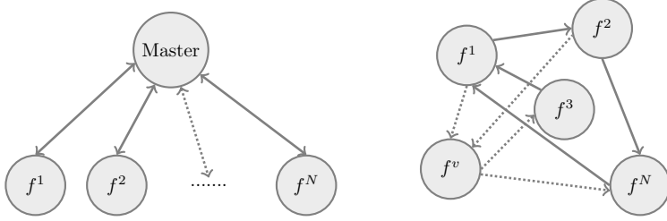
Figure 2.2: Distributed optimization setups: centralized versus decentralized.
