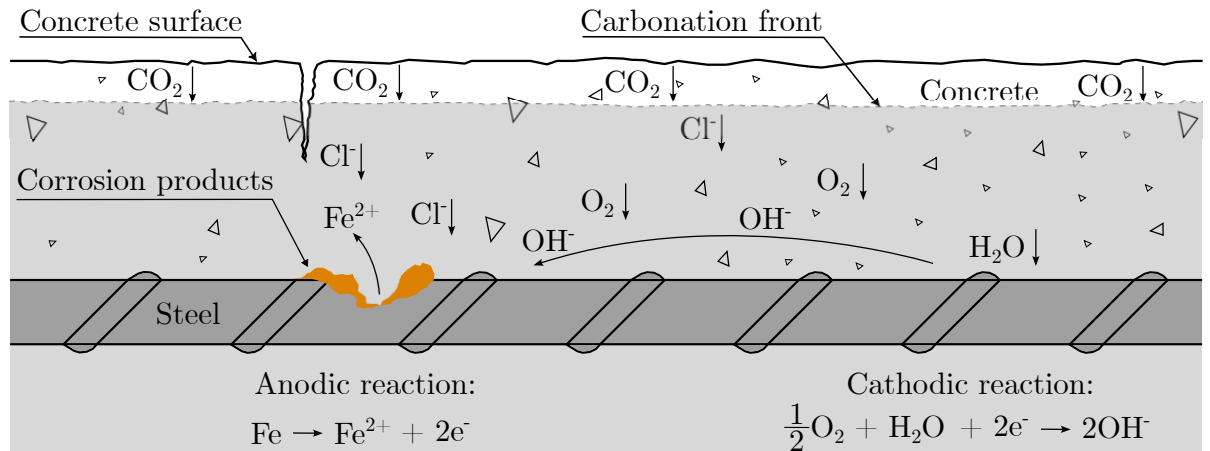
Figure 2.1: Illustration of corrosion of steel reinforcement in concrete.
