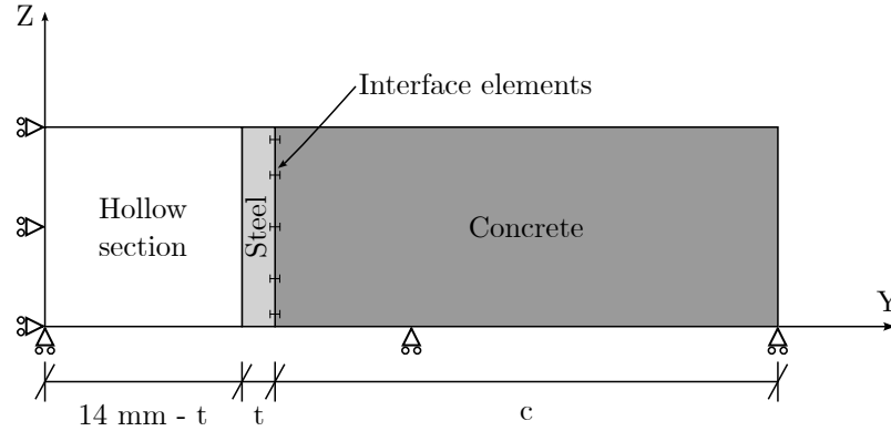
Figure 5.1: Axisymmetric model for parameter study on steel wall thickness ( t ) and concrete cover ( c ).
