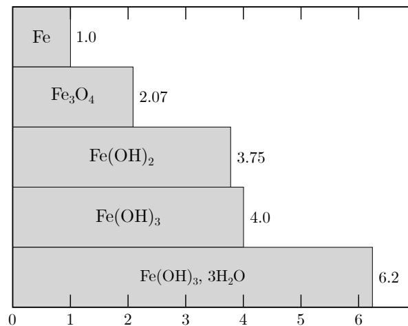
Figure 2.3: Volumetric ratio between various types of corrosion products and iron. Modified from [31].
