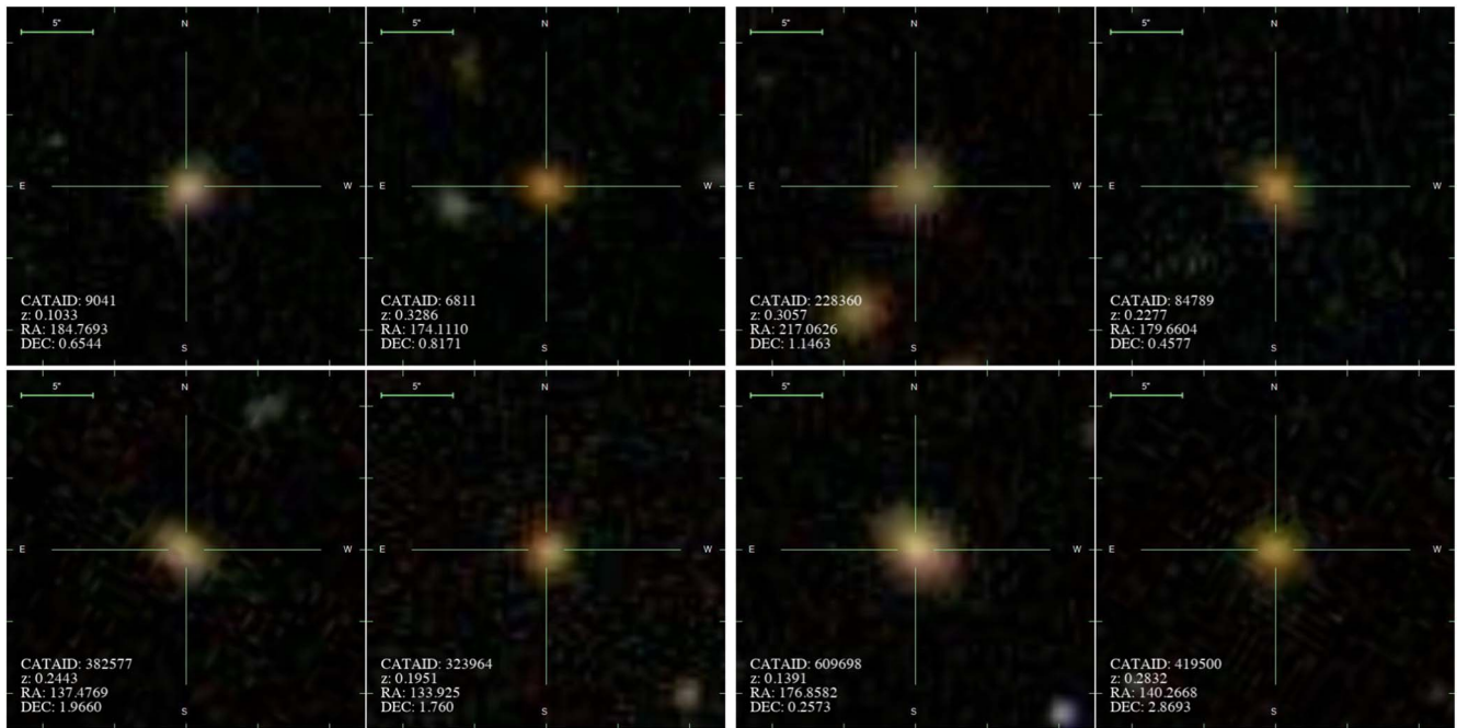
Figure 4. Comparison galaxy examples.
