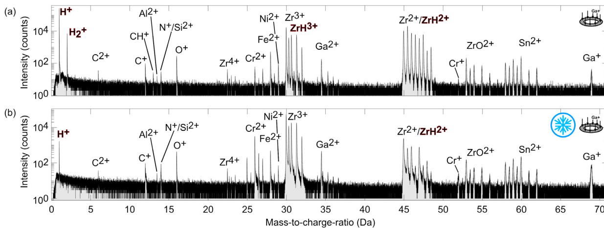
Fig. 2. Mass-to-charge spectra from two APT tips (both irradiated Alloy 2) measured in voltage pulsing mode. The spectrum in (a) stems from a tip that was sharpened at room temperature and analyzed at 70 K with a pulse fraction of 20%. The spectrum in (b) stems from a tip that was sharpened at -150^\circ\text{C} and measured at 90 K and pulse fraction of 15%. The ionic species used in the calculation of the hydrogen fraction are marked by red outlines.
