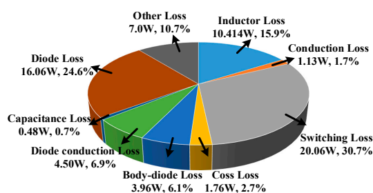
Figure 14. Power loss distribution of Boost PFC converter.
