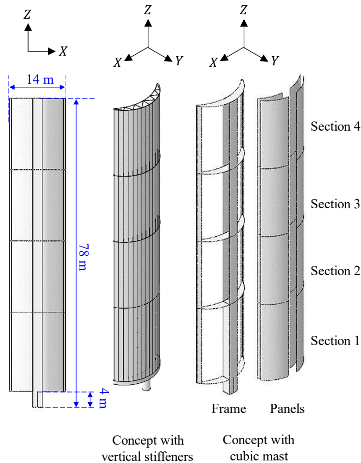
Figure 6. Size and structural designs of the wingsail.
