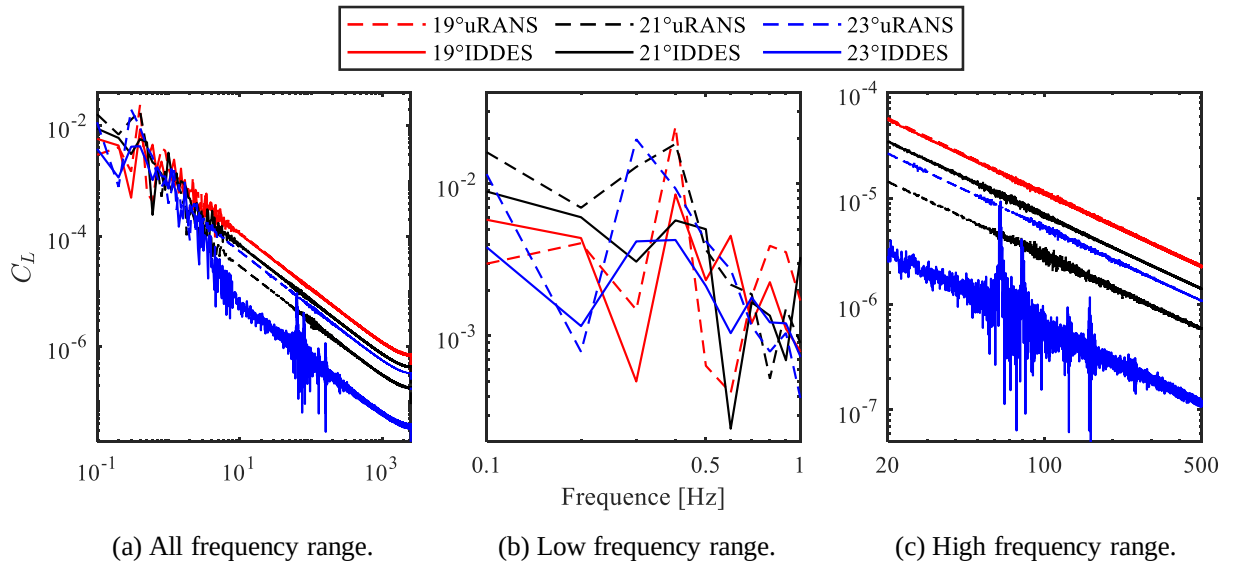
Figure 18. FFT results of C_L , fully expanded condition.
