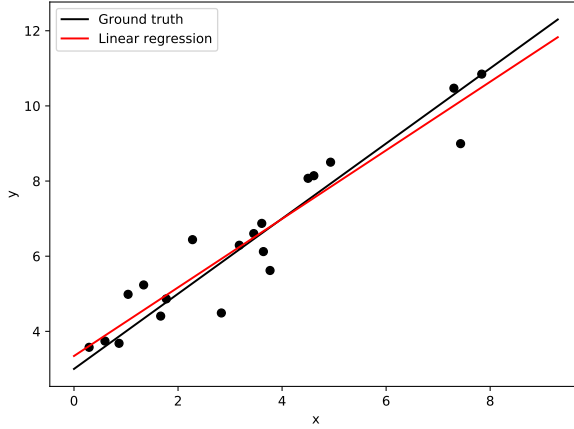
Figure 4.1: A line (red) is fitted to the noisy data (black dots).
