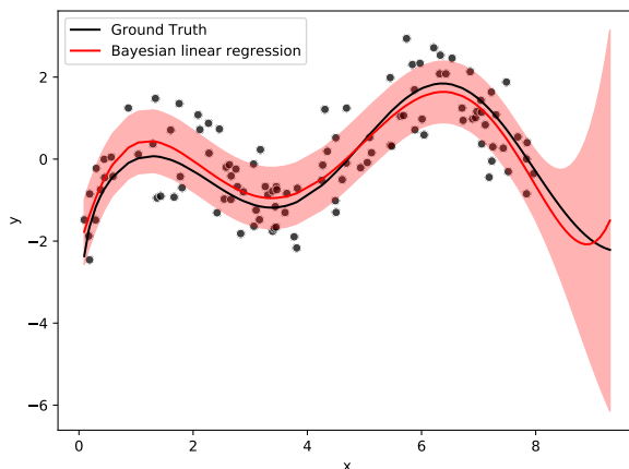
Figure 4.2: A 6^{th} order polynomial is fitted to noisy input data.
