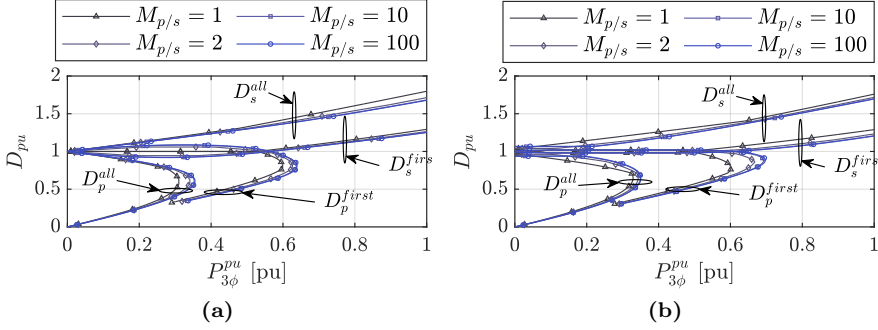
Figure 7.7: Effect of number of levels ( M_{p/s} = M_p = M_s ) on the turn-ON ZVS boundaries of a CTB-CTB-DAB converter with \tau_{p/s} = 10\% . (a) For the YY windings configuration. (b) For the Y\Delta configuration.
