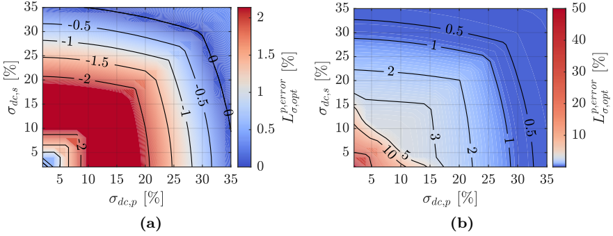
Figure 5.12: L_{\sigma, opt}^{p, error} (a) For the 3\phi -YY-DAB. (b) For the 3\phi -Y \Delta -DAB.
