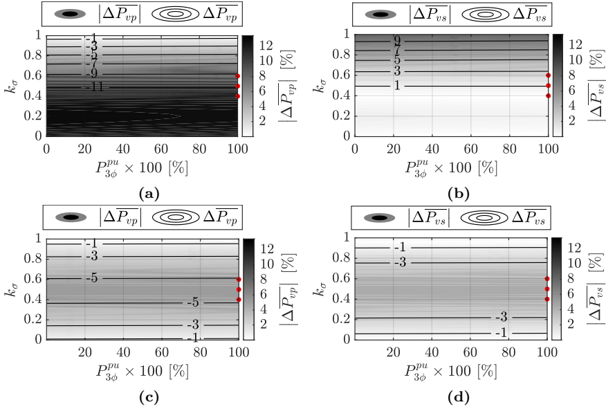
Figure 8.5: The estimation error of core loss density. (a) \Delta\overline{P}_{vp} for Y \Delta configuration. (b) \Delta\overline{P}_{vs} for Y \Delta configuration. (c) \Delta\overline{P}_{vp} for \Delta Y configuration. (d) \Delta\overline{P}_{vs} for \Delta Y configuration.
