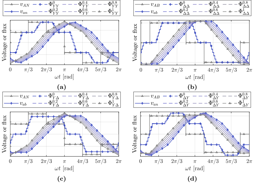
Figure 8.1: Phase voltages and flux waveforms, \Phi^{k_\sigma} , of a multilevel DAB converter at \varphi = \pi/6 for different values of k_\sigma . (a) YY configuration. (b) \Delta\Delta configuration. (c) Y \Delta configuration. (d) \Delta Y configuration.
