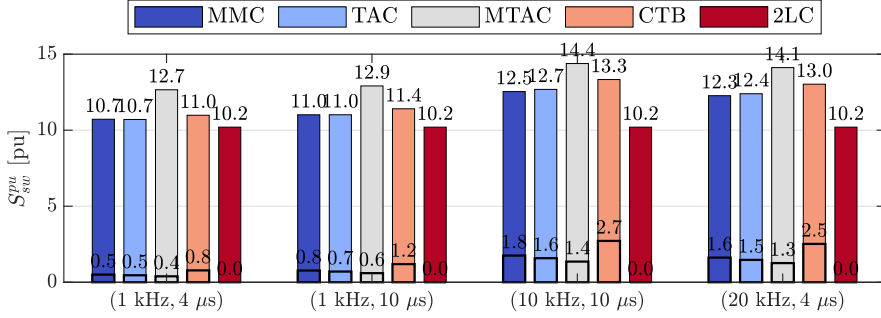
Figure 6.6: S_{sw,tot}^{pu} of the converters provided for ( f_{sw}, \tau ) pairs shown by (*) on Figure 6.2 and Figure 6.3 (the highlighted portions of the bars are the installed apparent power for the auxiliary switches).
