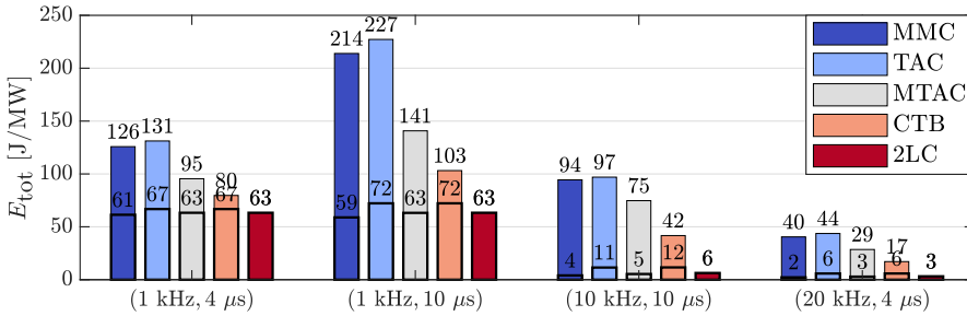
Figure 6.4: The energy storage requirement of the converters provided for (f_{\text{sw}}, \tau) pairs shown by (*) on Figure 6.2 and Figure 6.3 (the highlighted portions of the bars are the amount of energy required for the dc-links).
