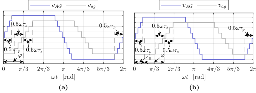
Figure 7.1: Reference P2G waveforms for ZVS calculations. (a) For YY-DAB. (b) For YΔ-DAB.
