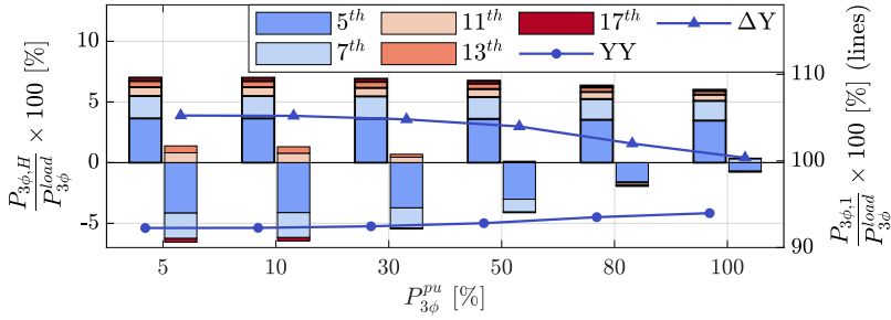
Figure 9.4: The active power transferred by each harmonic. The YY and \Delta Y are illustrated with bold and solid bars, respectively.
