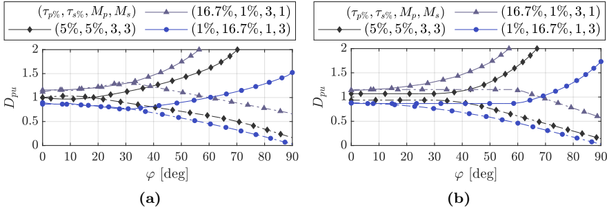
Figure 7.11: Comparison of the turn-ON ZVS boundaries obtained from simulations (shown by markers) and calculation for a CTB-CTB-DAB. (a) For the YY windings configuration. (b) For the Y \Delta windings configuration.
