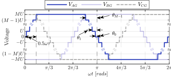
Figure 2.5: The P2G voltages of a 3\phi (2M + 1) -level converter; where \omega = 2\pi f_{sw} and f_{sw} is the switching frequency of the converter, M is the number of steps starting from zero in the positive direction in the waveform, \theta_k is the k th-step phase shift (where k \in \{0, \dots, M - 1\} ), U is the amplitude of each step and \tau is the transition time.
