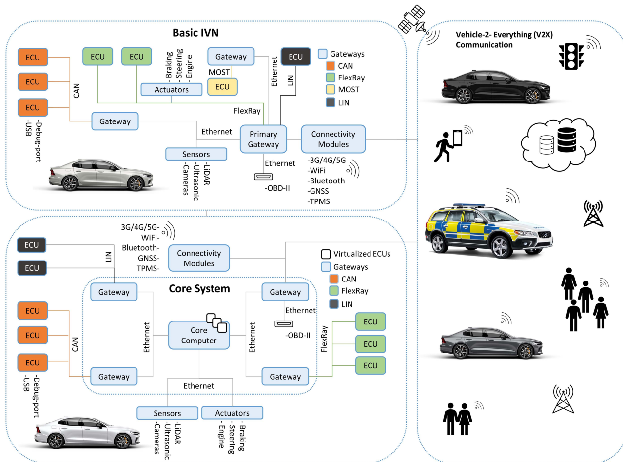
Fig. 1. The In-Vehicle Network and V2X Communication.
