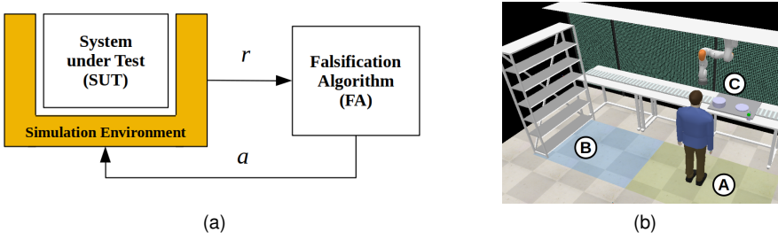
Figure 5.5: (a) The principle of simulation-based falsification: the falsification algorithm (FA) chooses actions a to adapt the simulation environment which excites the system under test (SUT) and receives rewards r (e.g. risk or coverage metrics). (b) The SUT used for testing the proposed automata constrained reinforcement learning: the nominal operating conditions are to walk from A to B to pick parts from the shelf, walk back, and assemble the parts in collaboration with the robot (C).
