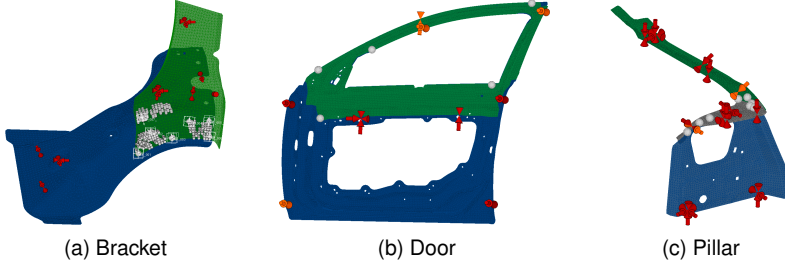
Figure 5.1: The three use cases for our experiments: (a) shows a sub-assembly of a car reinforcement bracket. Its two parts are positioned in space by twelve locators (shown in red). (b) shows the frame of a car door. Its two sheet metal parts are positioned in space by 19 locators. (c) shows a pillar of a car, consisting of three parts held in place by 20 locators. A digital twin computes the geometric quality after the assembly process (positioning, clamping, joining, releasing, scanning) based on several detailed Finite Element Method calculations, including elastic deformations and springback under the assembly forces. The final geometric quality may be influenced by adjusting each single locator along its axis.
