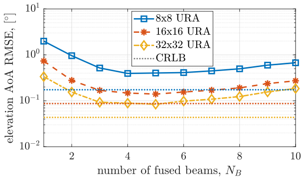
(a) RMSE of estimated elevation AoA as a function of total fused beams.
