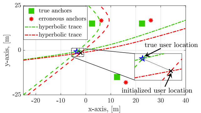
(a) User location initialization using the TDoA measurements based on erroneous anchor locations.
