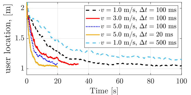
(b) RMSE of user location
