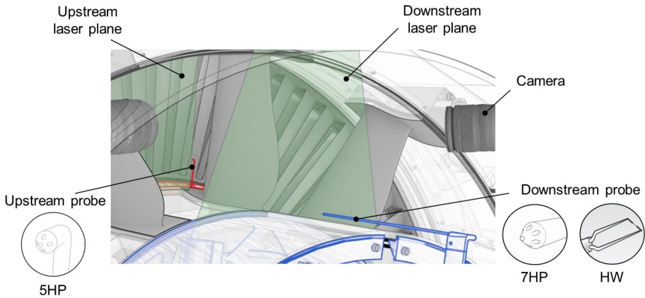
Figure 3: Isometric view of the test section with probes and laser planes located upstream and downstream OGVs for total pressure, HW and PIV measurements.
