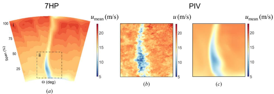
Figure 9: (a) Mean velocity distribution from the 7HP and PIV contours of (b) instantaneous and (c) mean velocity at the outlet plane.
