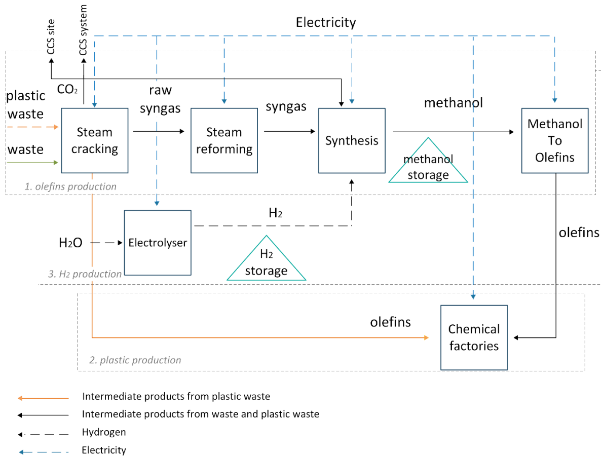
Figure 2.4: Schematic representation of the electrified plastics production process.
