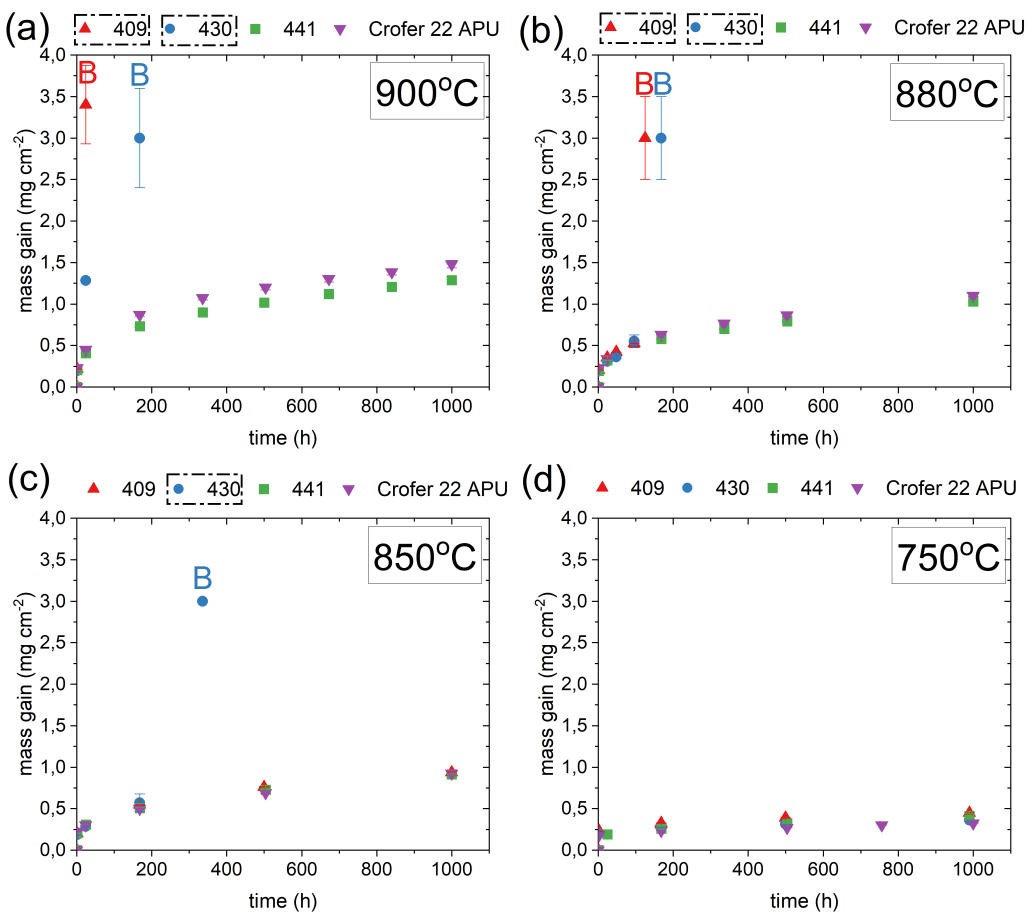
Figure 6.18: Mass gains of Ce/Co-coated AISI 409, AISI 430, AISI 441 and Crofer 22 APU exposed at temperatures in the range of 750°-900°C for 1,000 h in air + 3% H 2 O. The "B" indicates the time at which breakaway corrosion was observed.
