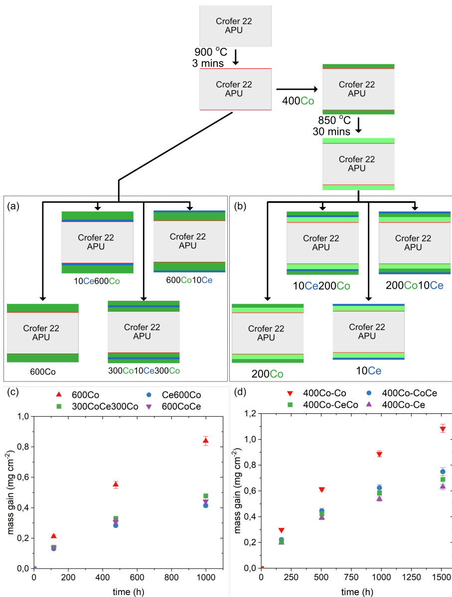
Figure 6.16: Fabricated coatings on pre-oxidised Crofer 22 APU (a) The four fabricated coatings are: 600 nm Co; 10 nm Ce + 600 nm Co; 300 nm Co + 10 nm Ce + 300 nm Co; and 600 nm Co + 10 nm Ce. (b) On four additional sheets of pre-oxidised Crofer 22 APU, 400 nm Co was deposited and then exposed to 850°C for 30 minutes to oxidise the Co to Co 3 O 4 . The four fabricated coatings are: 200 nm Co; 10 nm Ce + 200 nm Co; 200 nm Co + 10 nm Ce; and 10 nm Ce. (c,d) Mass gains of the coated steels in (a), and (b) exposed to 850°C in air + 3% H 2 O. Mass gain due to oxidation of metallic Co is subtracted from subsequent data before plotting.
