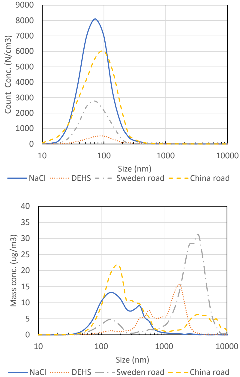
Figure 24 Outside air particle size distribution of count concentration ( \text{N}/\text{cm}^3 ) and mass concentration ( \mu\text{g}/\text{m}^3 ). Examples of the generated dust of DEHS, NaCl, road air in Sweden 2022 and China 2019 are compared. Four examples all have \text{PM}_{2.5} concentration around 100 \mu\text{g}/\text{m}^3
