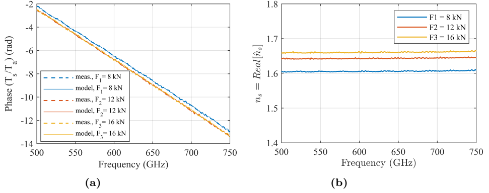
Figure 5.2: a) Phase of relative transmission for tablets (experiment number 2 in table four chapter three with three different compaction forces, F_1 = 8 kN, F_2 = 12 kN, F_3 = 16 kN, showing good agreement between model and measurement data b) Real part of effective refractive index over frequency. A higher compaction force increased the effective refractive index.
