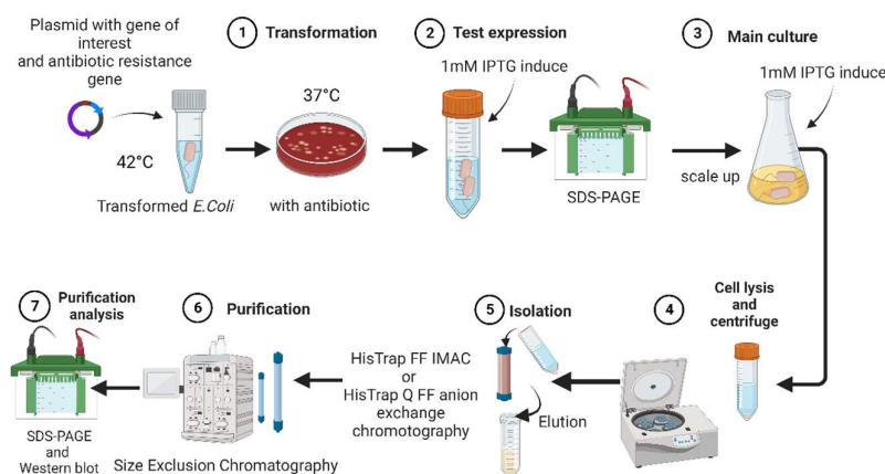
Figure 6. Memo1 and Atox1 recombinant proteins are produced using an E. coli as expression host [111]. After transformation, colonies are screened for expression analysis. A single colony is picked and grown with their respective antibiotics. Small test expressions are carried out to optimize and determine the solubility and yield of the protein of interest. The process is then scaled up where 1/100 of an overnight grown culture dilution cells are grown at 37°C, induced at O.D of 0.6-0.8, and grown at 20°C overnight post-induction. The cells are pelleted by centrifugation, lysed, and the protein's supernatant is then subjected to different chromatography techniques to isolate and purify the protein of interest. Finally, the purified protein is checked for purity and homogeneity using size exclusion, SDS-PAGE and western blot, respectively.
