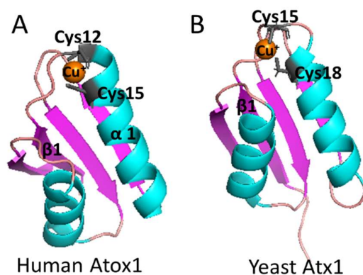
Figure 2. Crystal structures of Atox1 homolog. (A) Human CuAtox1 (1FEE); (B) Yeast CuAtx1 (1FD8). \alpha helices in blue, \beta strands in magenta, loop regions in pink. Atox1 CXXC motif are displayed as grey stick. Cu ions (orange spheres).
