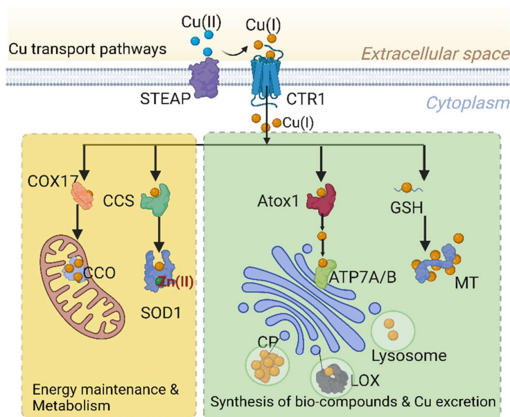
Figure 1. Overview of systemic and cellular Cu homeostasis. Once Cu(II) is reduced to Cu(I) by proteins from the STEAP family, Cu is transported into intracellular through the CTR1. From there, Cu is transferred to chaperones CCS, COX17, and ATOX1, distributing it to various destinations, including cytosolic SOD1 and CCO in the mitochondria, ATP7A/B at TGN. Cu binds to MT and GSH, which act as cellular antioxidants and prevent ROS formation. Within the TGN, Cu is incorporated into Cu-dependent enzymes, such as lysyl oxidase (LOX), which are transported through the secretory pathway. When excess Cu enters cells, ATP7A can also secrete Cu into the extracellular space. Created with BioRender.com .
