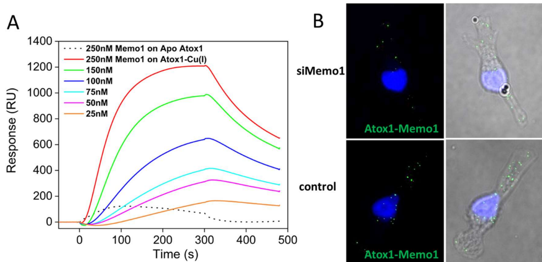
Figure 18. Investigation of Memo1-Atox1 potential interaction (A) Memo1 titration to Cu(I)-loaded Atox1 by SPR (solid curves). Memo1 injected onto to apo-Atox1 surface (dashed curve). (B) Confocal microscopy images of Memo1-Atox1 proximity in Memo1 knockdown (upper panel) and control (lower panel) MDA-MB 231 cells using PLA. Left panel: confocal fluorescence images; Right panel: overlay of the confocal fluorescence images with the bright field images. (blue=DAPI, indicating nucleus; green=PLA dots)
