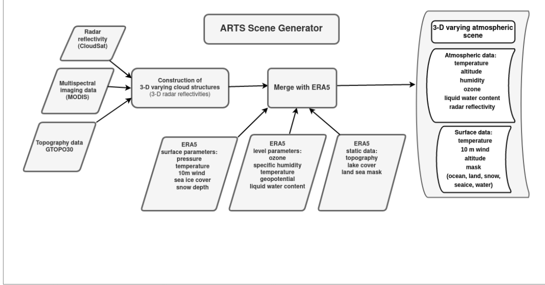
Figure 1: Flowchart summarising the input data, processes, and outputs of the scene generation scheme. The complete algorithm has been implemented within a Python toolbox denoted as the ARTS Scene Generator.
