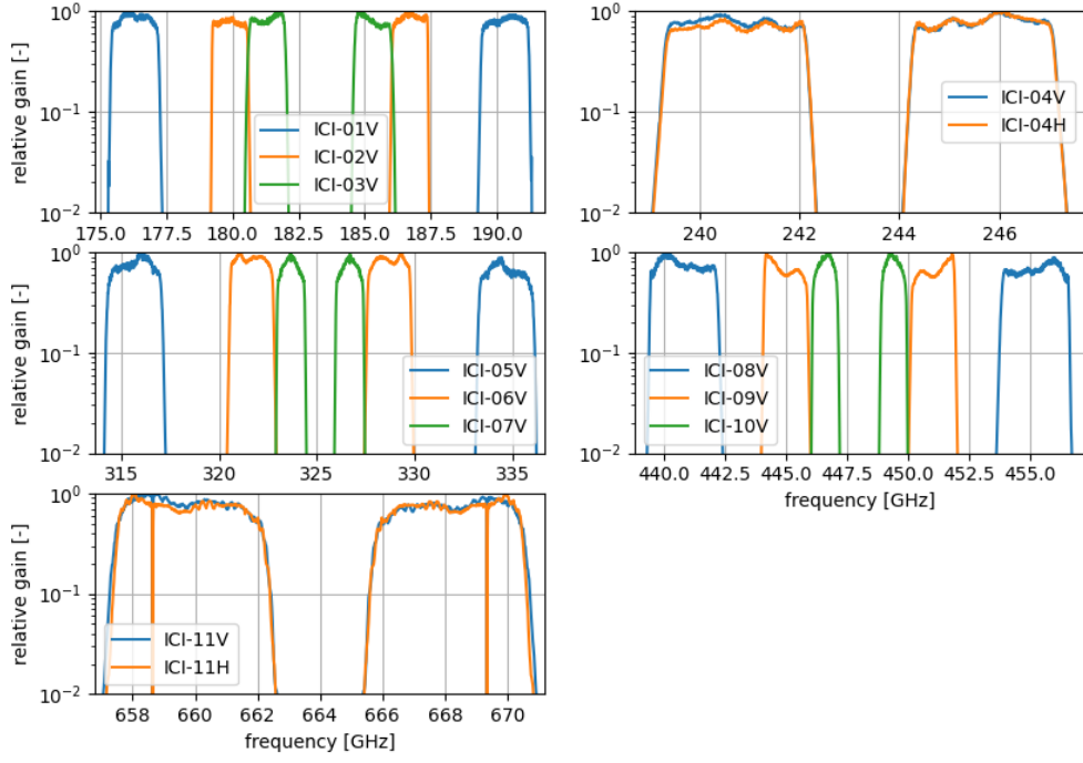
Figure 17: Spectral response function of the 13 ICI channels.
