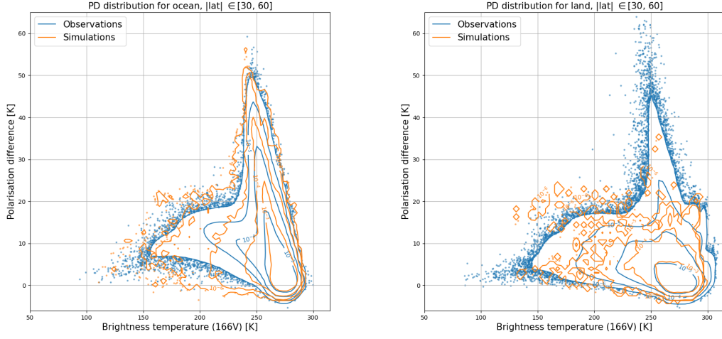
Figure 37: Joint probability distributions of polarisation difference (PD) and brightness temperature for the 166V channel ( T_{b,166V} ) for ocean (left) and land (right) at mid-latitudes in the range -60 to -30 and 30 to 60 degrees. Contour lines of the probability distributions for observations (blue) and simulations (orange) are seen at levels 10^{-6} \text{ K}^{-2} , 10^{-5} \text{ K}^{-2} , 10^{-4} \text{ K}^{-2} and 10^{-3} \text{ K}^{-2} . A random sample of 1% of the simulated data points with lower probability than 10^{-6} \text{ K}^{-2} are plotted as blue dots. For the simulations all points with lower probability than 10^{-6} \text{ K}^{-2} are plotted as orange dots.
