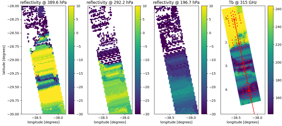
Figure 6: The three panels to the left shows radar reflectivity at three different pressure levels. The right panel shows simulated brightness temperatures at a frequency of 315 GHz. The simulation was done by dividing the scene into 4 smaller sub-scenes (denoted by numbers 1 to 4 in the right panel). The red markers around the center position of each smaller scene indicates the position of a subset of pencil beam simulations, used to generate the plots found in Figure 7. The red line from the center position of scene 1 points in the direction towards the sensor.
