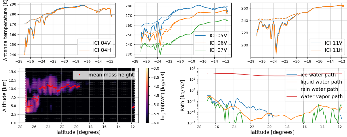
Figure 4: The upper panels show antenna temperature for seven of the ICI channels for a simulation based on the cloud structure displayed in Figure 2. The lower panel shows the underlying cloud, rain, and water vapour properties of the volume sampled by the simulated observation.
