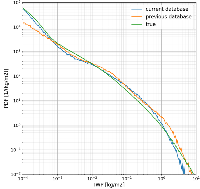
Figure 19: Retrieved (posterior median value) and true probability density function of IWP, for the data displayed in Figure 18.
