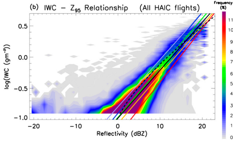
Figure 5: The distribution of joint IWC and dBZ measurements, as available from Protat et al. (2016).
