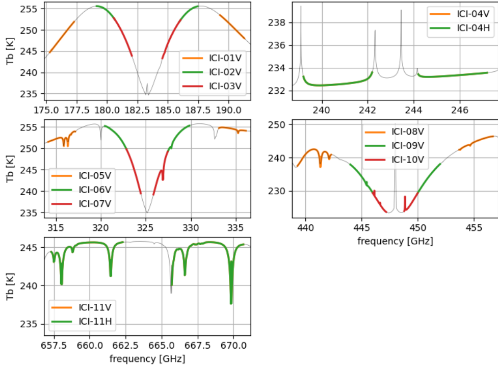
Figure 18: Simulated brightness temperature as function of frequency for one scene of the ERESMAA dataset.
