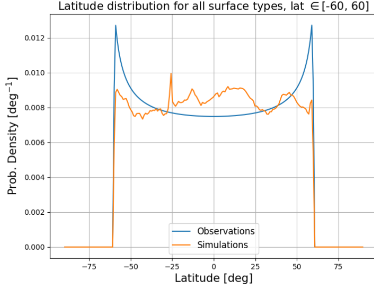
Figure 28: Latitude probability distributions for all surface types and latitudes in the range -60 degrees to 60 degrees.
