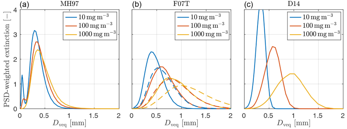
Figure 3: Normalised extinction as function of volume equivalent diameter ( D_{\text{veq}} ) for three different particle size distributions. Figure from Ekelund et al. (2020).
