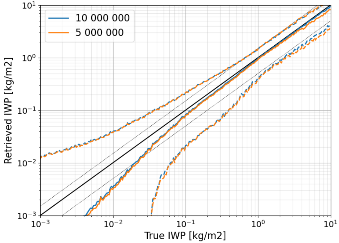
Figure 26: Estimated retrieval performance for IWP using a retrieval database consisting of around 10 and 5 million states. The solid lines show the median of the retrieved posterior median values, and the dashed lines show the median of the retrieved 5th and 95th percentile.
