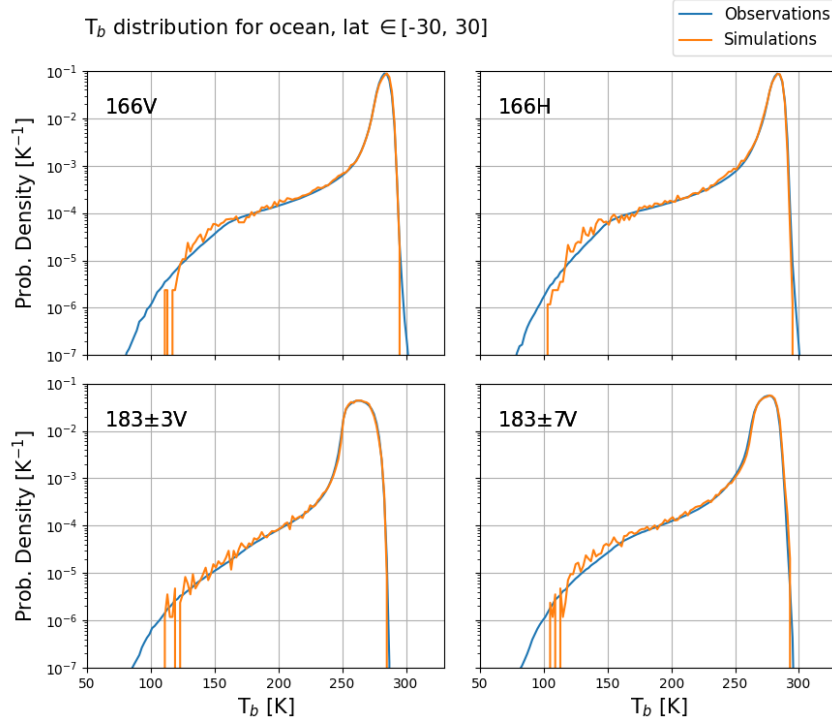
Figure 31: Brightness temperature ( T_b ) probability distributions for each of the high-frequency channels of GMI for ocean at tropical latitudes, i.e. only data from latitudes -30 to 30 are included.
