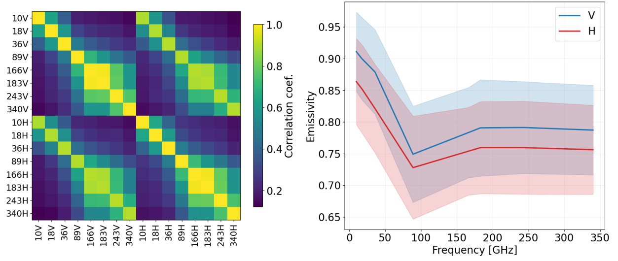
Figure 15: (left) The correlation matrix for snow-covered surface type, and (right) the mean emissivities and standard deviation.
