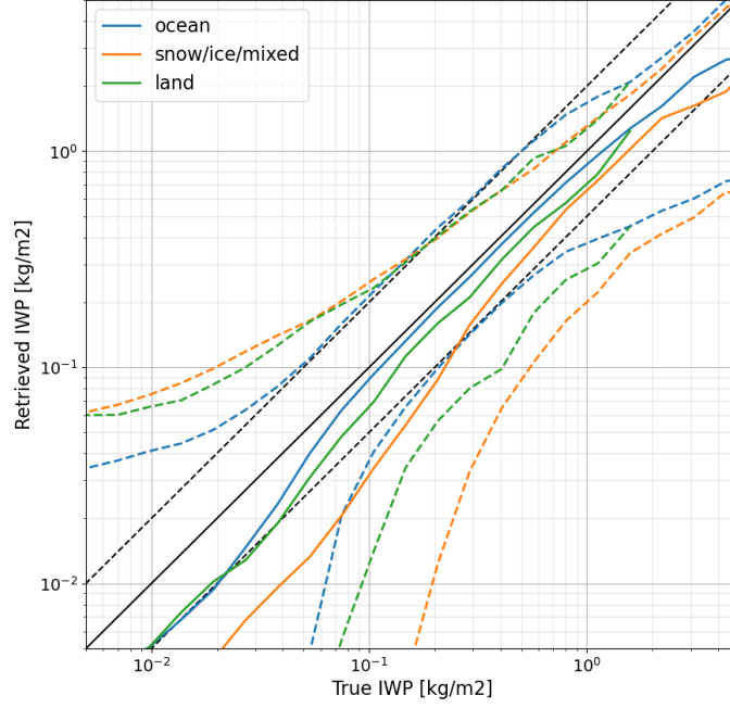
Figure 23: Estimated retrieval performance for IWP and for a surface temperature lower than 0^{\circ}\text{C} and for different surface types. The performance for snow ice, and mixed surface types were similar and combined to result in a less noisy plot. The solid lines show the median of the retrieved posterior median values, and the dashed lines show the median of the retrieved 5th and 95th percentile.
