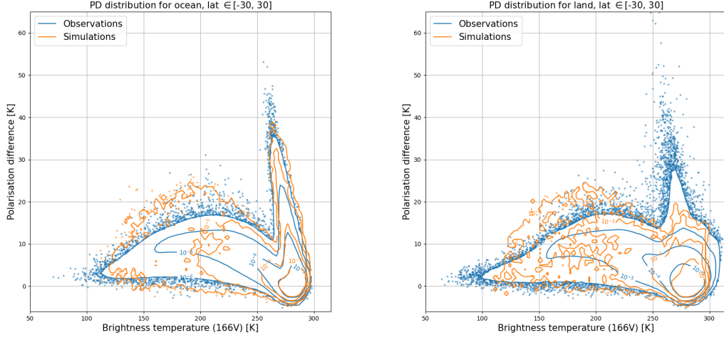
Figure 36: Joint probability distributions of polarisation difference (PD) and brightness temperature for the 166V channel ( T_{b,166V} ) for ocean (left) and land (right) at tropical latitudes in the range -30 degrees to 30 degrees. Contour lines of the probability distributions for observations (blue) and simulations (orange) are seen at levels 10^{-6} \text{ K}^{-2} , 10^{-5} \text{ K}^{-2} , 10^{-4} \text{ K}^{-2} and 10^{-3} \text{ K}^{-2} . A random sample of 1% of the simulated data points with lower probability than 10^{-6} \text{ K}^{-2} are plotted as blue dots. For the simulations all points with lower probability than 10^{-6} \text{ K}^{-2} are plotted as orange dots.
