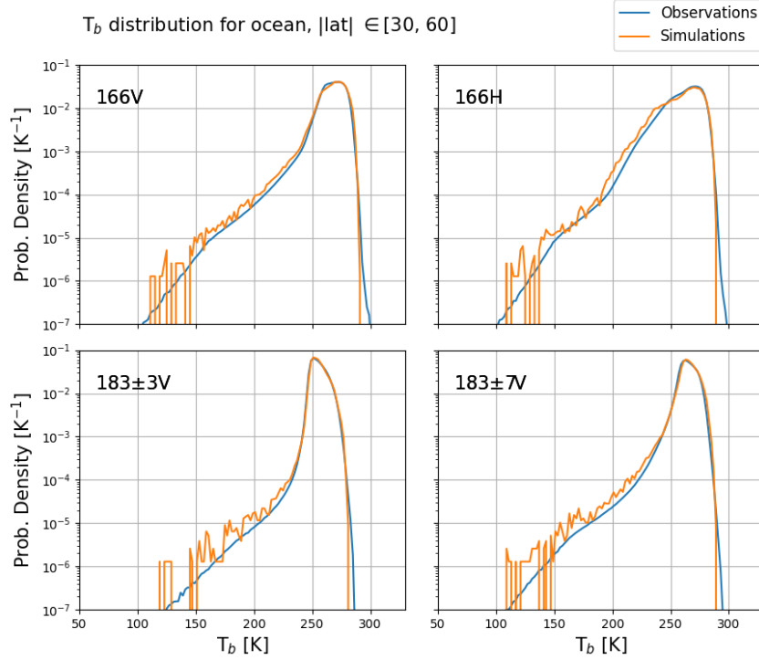
Figure 33: Brightness temperature ( T_b ) probability distributions for each of the high-frequency channels of GMI for ocean at mid-latitudes i.e. only data from latitudes -60 to -30 and 30 to 60 are included.
