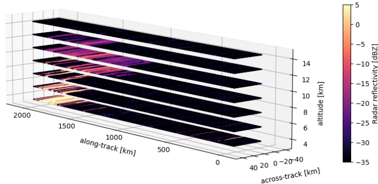
Figure 2: Example of a generated 3D varying radar reflectivity field.
