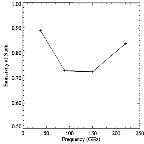
Figure 7. Nadir emissivity versus frequency on May 20, 1998.
