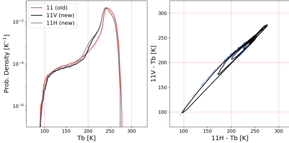
Figure 4: A comparison of the 664 GHz channel T_b distributions from the previous database and the new database (left). Only one distribution is available from the old database. This is denoted as 11 in the plot and denotes the intensity simulation computed as the mean of 11V and 11H. 11H and 11V are available from the new database and both are plotted in comparison to the old database. The two-dimensional distribution between 11V and 11H is also shown (right), where the blue markers indicate samples that occur with a probability density less than 10^{-6} K^{-2} .
