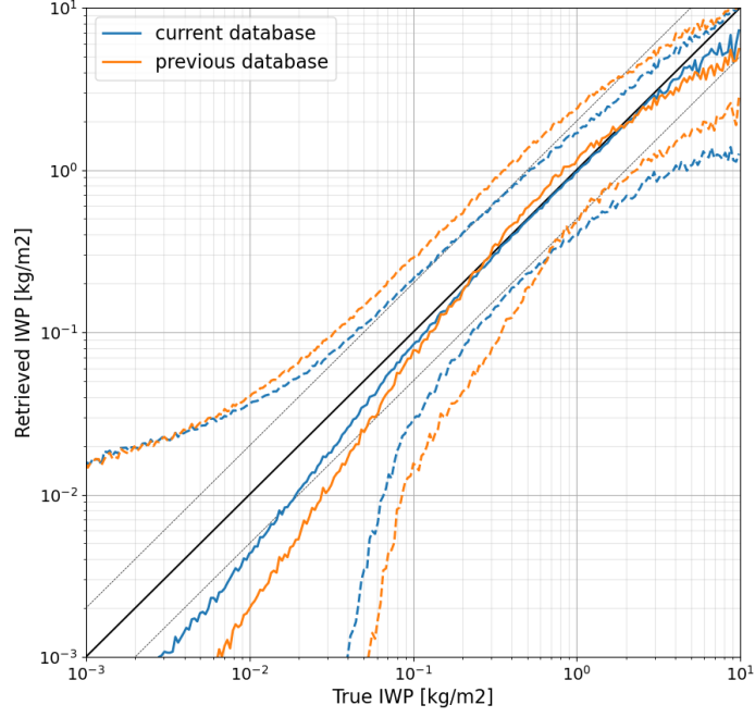
Figure 18: Estimated retrieval performance for IWP using the current and previous database and for mixed climatic conditions. The solid lines show the median of the retrieved posterior median values, the colored dashed lines show the median of the retrieved 5th and 95th percentile.
