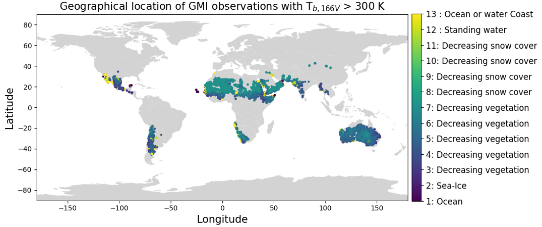
Figure 11: Geographical location of GMI observations with measured T_b > 300 K for the 166V channel. The GPROF surface classifications of the observations are indicated by the colorbar. Decreasing vegetation 3-7 are the classifications used for surface type 'land'.
