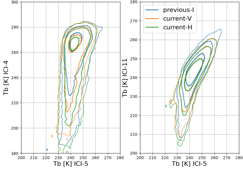
Figure 17: Contour plots comparing distribution of simulated observations associated to the previous and current database for the ICI-04, ICI-05, and ICI-11 channels. The current database contains data for both the V and H channels for ICI-04 and ICI-11, while the previous database only contains intensity simulation (mean of V and H). Three contour lines (0.0001 , 0.001, 0.01) are displayed.
