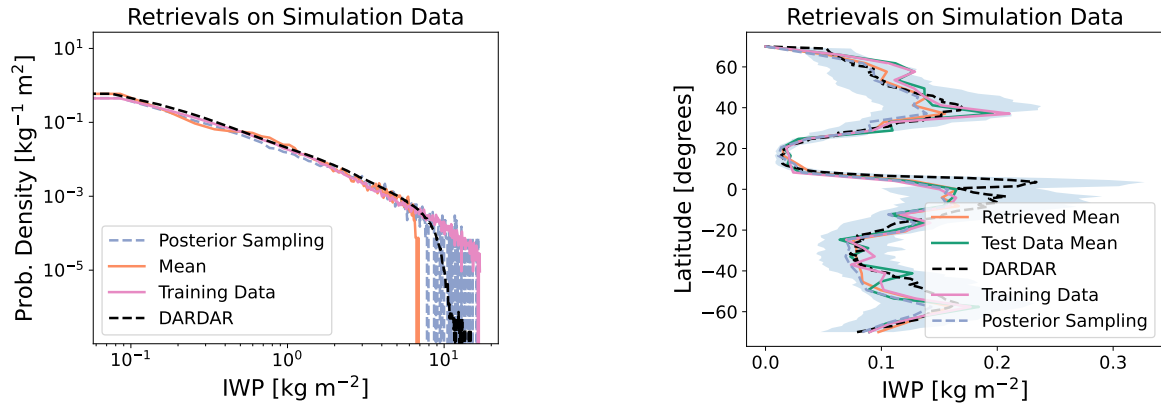
Figure 12: A comparison of (left) PDFs and (right) the zonal means of retrieved IWP using the test GMI database.
