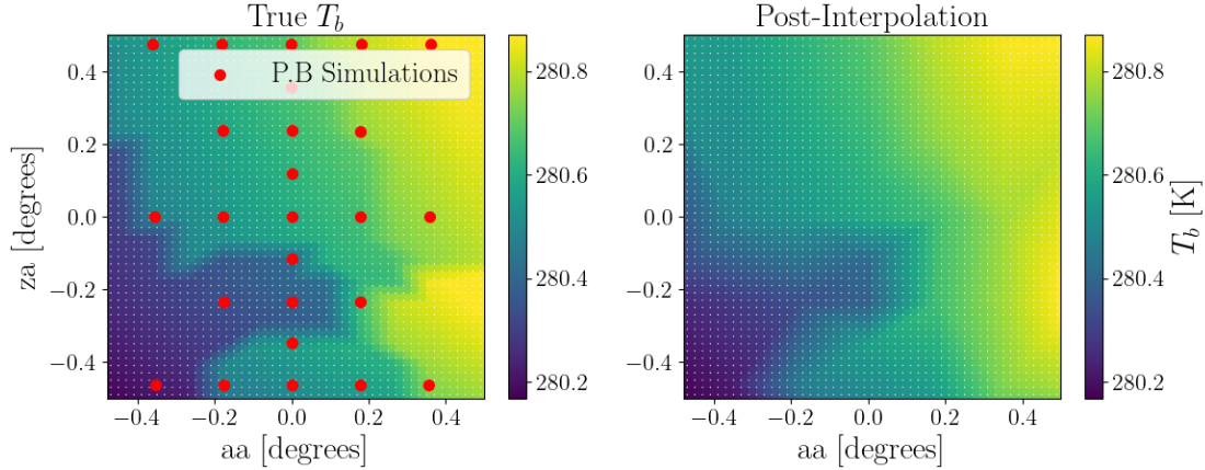
Figure 7: Both panels show brightness temperatures as function of relative zenith and azimuth angles. The red markers in the left panel are positions of pencil beam simulations, where the centre marker is the point at which the boresight of the antenna is pointed towards. A positive zenith and azimuth angle corresponds to a position below and to the right of the antenna boresight direction. The right panel shows the data re-gridded onto the positions of the ICI-01V antenna pattern grid through the use of interpolation, as described in step 3 of the antenna temperature procedure described above. The brightness temperatures in the left panel, denoted ‘True’, were obtained by running simulations on each grid point. They are included in the figure to act as a comparison to the interpolated temperatures.
