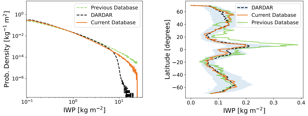
Figure 6: A comparison of (left) PDFs and (right) the zonal means of IWP values from the current cloud radiation retrieval database, the previous database, and IWP values from the DARDAR product. The shaded region shown for the zonal means (right) represents the \pm 40\% uncertainty in DARDAR IWP. DARDAR data are taken for all months in 2010. Distributions were calculated across all latitudes and surface types available.
