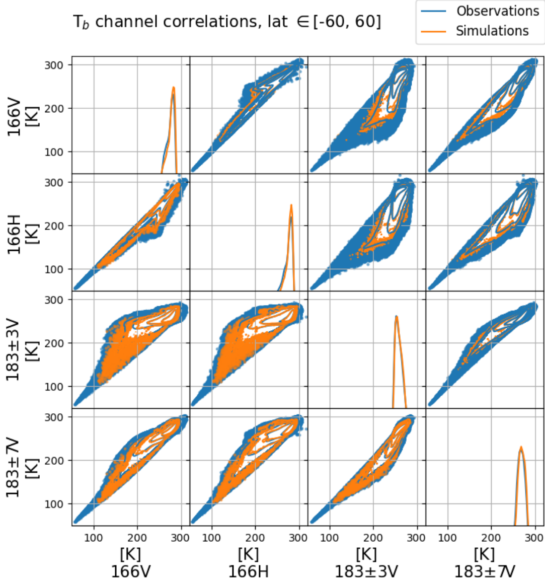
Figure 9: Brightness temperature ( T_b ) channel correlations for GMI observations (blue) and GMI simulations (orange). Joint probability distributions between each of the channels are seen where data from all surface types and from latitudes in the range -60 degrees to 60 degrees are used. Simulations are plotted on top of observations below the diagonal and above the diagonal, observations are plotted on top of simulations. The contour lines are at levels 10^{-6} \text{ K}^{-2} , 10^{-5} \text{ K}^{-2} , 10^{-4} \text{ K}^{-2} and 10^{-3} \text{ K}^{-2} and data points outside the 10^{-6} \text{ K}^{-2} contour are plotted as dots. Marginal distributions are seen at the diagonal.
