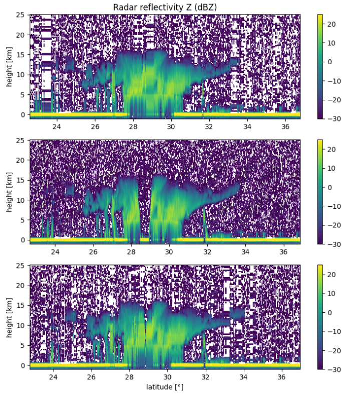
Figure 10: Continued from Figure 9, showing ‘Barkerized’ data for the scene in Figure 8. The figure shows constructed 2-D cross-sections of radar reflectivity along the westernmost, center, and easternmost path of the scene.
