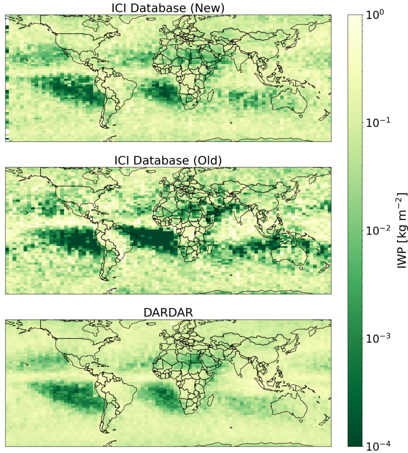
Figure 7: Global mean IWP from the new cloud radiation retrieval database (upper), the old database (middle), and the DARDAR product (lower). DARDAR data are taken for all months in 2010. Grid boxes span 2 degrees longitude by 2 degrees latitude.
