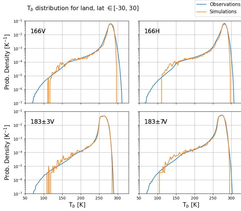
Figure 30: Brightness temperature ( T_b ) probability distributions for each of the high-frequency channels of GMI for land at tropical latitudes, i.e. only data from latitudes -30 to 30 are included.
