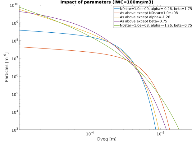
Figure 4: The impact of three parameters: N_0^* , \alpha and \beta on the variability of D14.
