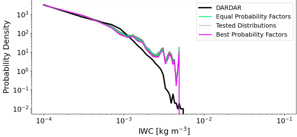
Figure 13: Distribution of IWC at an altitude of 8 km. \sim 10^5 distributions were tested. The distribution shown in green was obtained using all p_i = 1/6 , which was the default setting before improvements were implemented. The ‘best’ distribution, shown in pink, fails to perfectly match the DARDAR distribution at high IWC values due to lower limits currently set on the probability factors. However, the DARDAR distribution also contains relatively high levels of uncertainty and must not be taken as the truth. It must also be noted that this discrepancy occurs at low probability density values.
