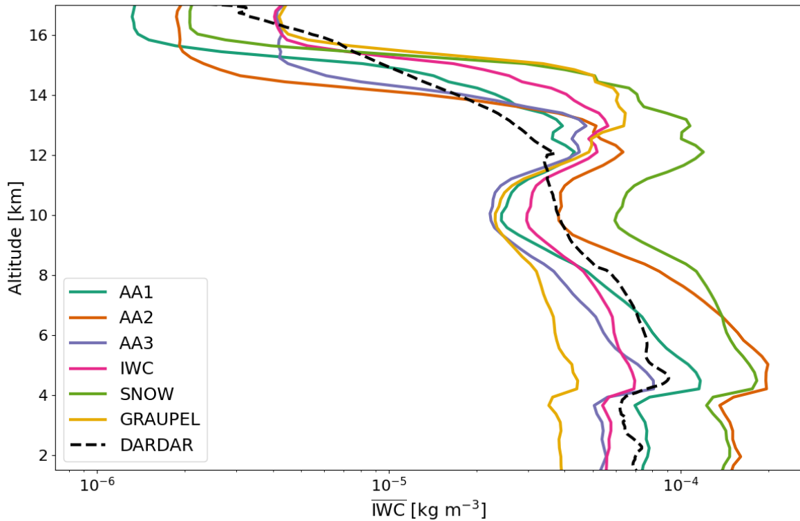
Figure 11: Mean IWC values obtained across the altitude grid. The mean was calculated over \sim 1000 simulations per particle model . DARDAR IWC values shown are mean IWC values for global, year-round (2010) data.
