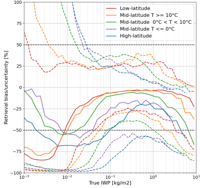
Figure 22: As Figure 21 but showing the performance in terms of a relative error and the dashed lines show data associated to the retrieved 16th and 84th percentile.
