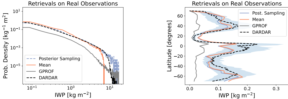
Figure 14: A comparison of (left) PDFs and (right) the zonal means of retrieved IWP from actual GMI observations.
