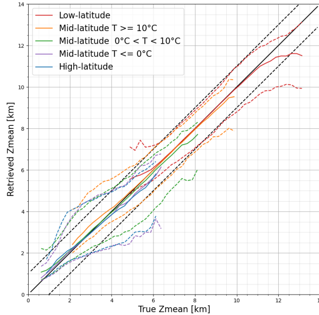
Figure 25: Estimated retrieval performance for Z_{\text{mean}} and five climatic regions. The solid lines show the median of the retrieved posterior median values, and the dashed lines show the median of the retrieved 5th and 95th percentile. Only data with a true IWP above 0.02 \text{ kg/m}^2 are used for low-latitude and warm mid-latitude, above 0.05 \text{ kg/m}^2 for intermediate warm mid-latitude, above 0.06 \text{ kg/m}^2 for cold mid-latitude, and above 0.1 \text{ kg/m}^2 for high-latitude.
