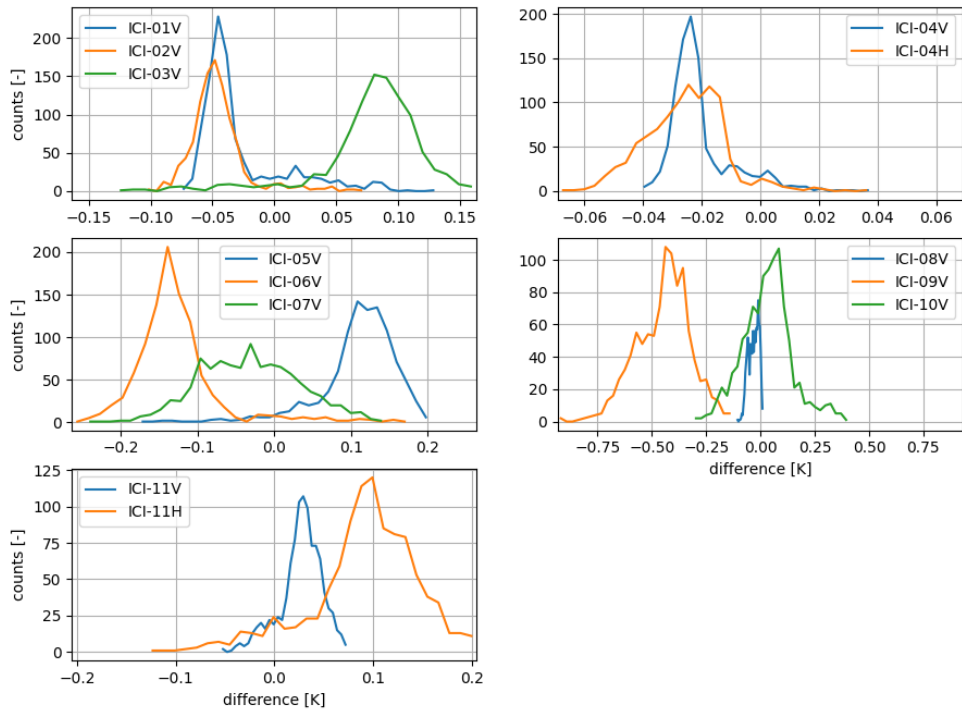
Figure 19: Histogram of brightness temperature differences due to neglecting the spectral response function for 1000 scenes of the ERESMAA dataset.
