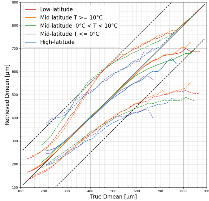
Figure 24: Estimated retrieval performance for Dmean and five climatic regions. The solid lines show the median of the retrieved posterior median values, and the dashed lines show the median of the retrieved 5th and 95th percentile. Only data with a true IWP above 0.02 \text{ kg/m}^2 are used for low-latitude and warm mid-latitude, above 0.05 \text{ kg/m}^2 for intermediate warm mid-latitude, above 0.06 \text{ kg/m}^2 for cold mid-latitude, and above 0.1 \text{ kg/m}^2 for high-latitude.
