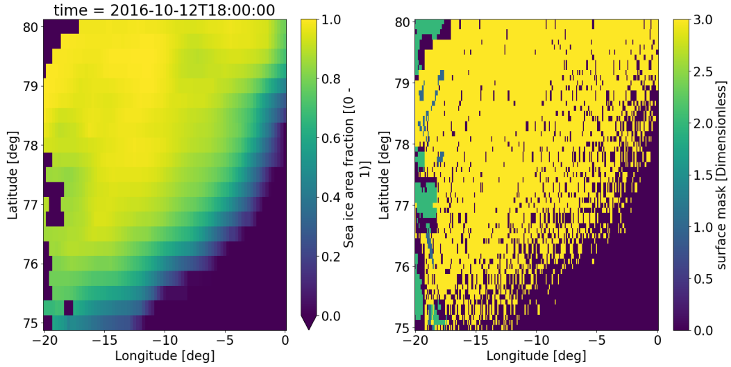
Figure 14: Sea ice concentrations up-scaled to 5 minute ( \sim 8 km) resolution.
