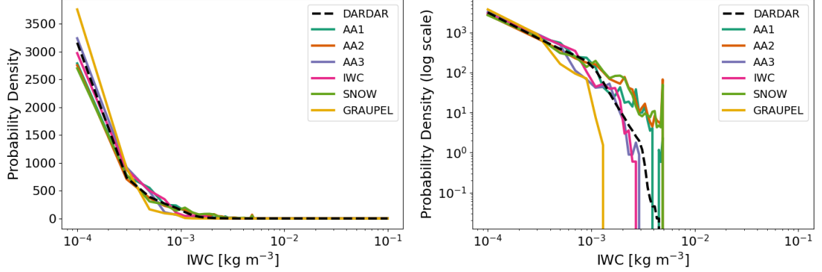
Figure 12: Distribution of IWC at an altitude of 8km. The plot on the right hand side shows the same distributions as the plot on the left, but with the probability density given on a log scale.
