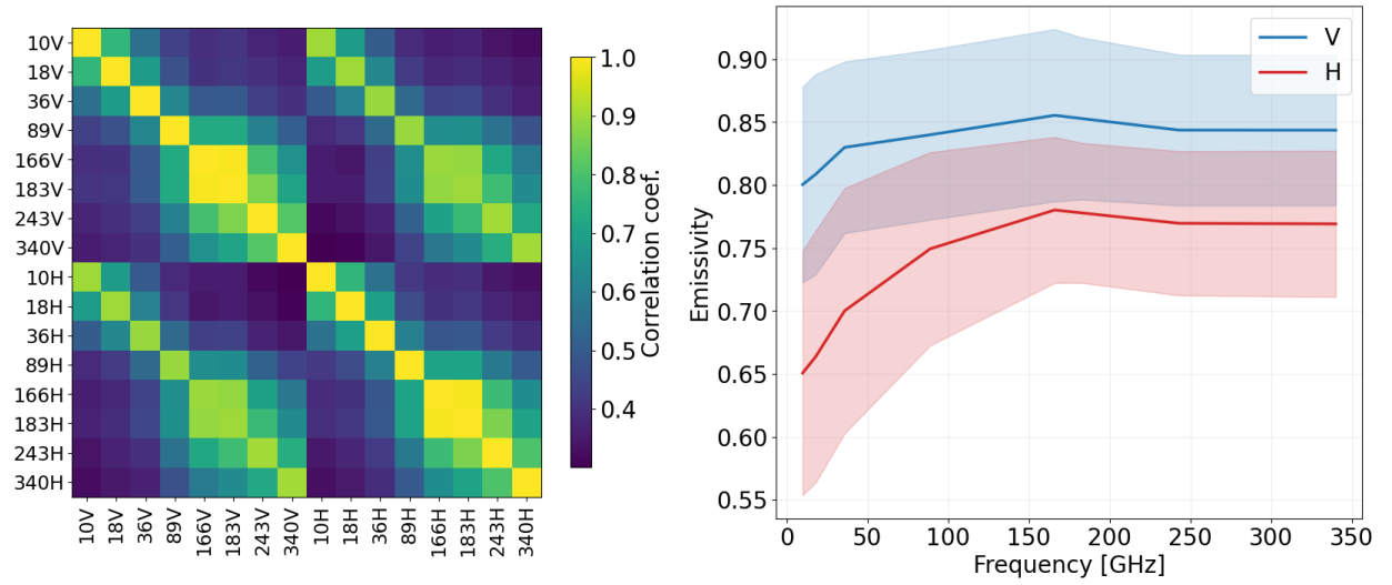
Figure 16: (left) The correlation matrix for sea ice surface type, and (right) the mean emissivities and standard deviation.
