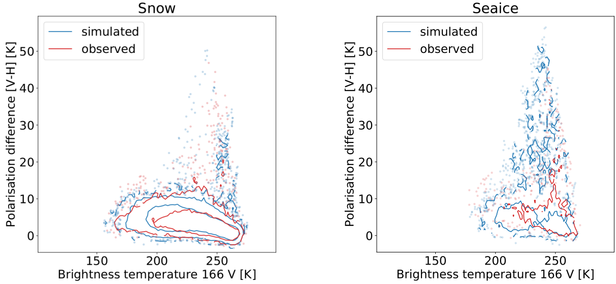
Figure 1: Polarisation difference contours ( 166V - 166H ) as a function of 166V GHz brightness temperatures ( T_b ) for observed GMI data (red) and simulated values (blue) over snow-covered land (left) and sea ice (right).
