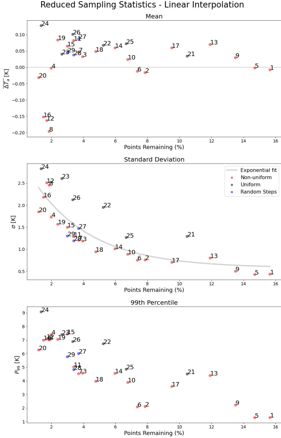
Figure 20: The mean, standard deviation, and 99th percentile of \Delta T_a , defined as the difference between values of T_a computed using reduced track settings and full track settings. Each numbered point refers to a pattern, defined as a track setting configuration. Statistics were computed over 100 atmospheric scenes, 3 sensor positions, and 4 channels, producing 1200 samples in total for each pattern . The standard deviation appears to exponentially increase with a decrease in number of points in a pattern.
