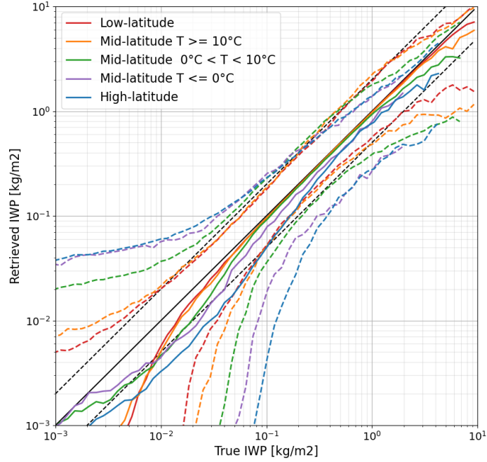
Figure 21: As Figure 20, but showing the data for a somewhat different IWP range.
