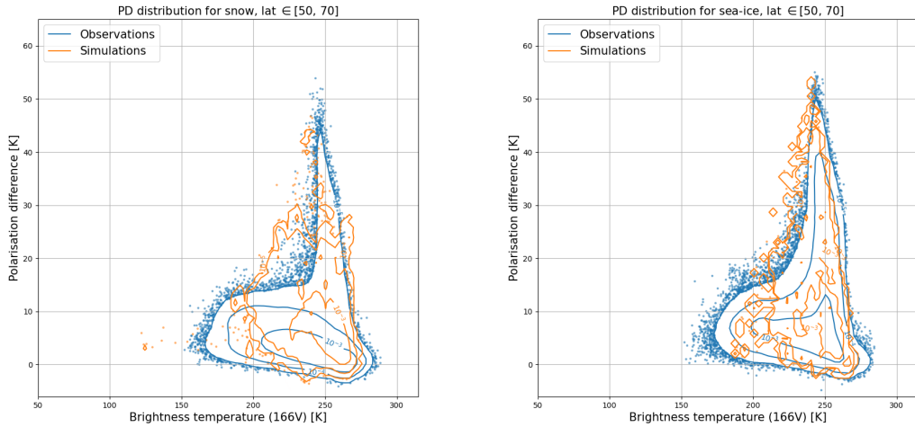
Figure 38: Joint probability distributions of polarisation difference (PD) and brightness temperature for the 166V channel ( T_{b,166V} ) for snow (left) and sea-ice (right) at northern-latitudes in the range 50 to 70 degrees. Contour lines of the probability distributions for observations (blue) and simulations (orange) are seen at levels 10^{-5} \text{ K}^{-2} , 10^{-4} \text{ K}^{-2} and 10^{-3} \text{ K}^{-2} . A random sample of 1% of the simulated data points with lower probability than 10^{-5} \text{ K}^{-2} are plotted as blue dots. For the simulations all points with lower probability than 10^{-5} \text{ K}^{-2} are plotted as orange dots. There are only about 42 000 cases in the simulation dataset for snow and only about 5000 cases in the simulation dataset for sea-ice.
