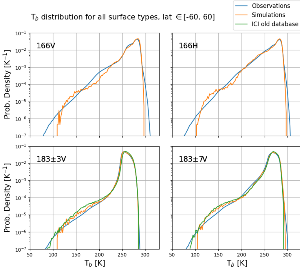
Figure 8: Brightness temperature ( T_b ) probability distributions for each of the high-frequency channels of GMI. Data from all surface types are used and from latitudes in the range -60 degrees to 60 degrees. Distributions for observations (blue) and simulations (orange) are seen for each channel and for the 183GHz channels, ICI T_b distributions for the old (preliminary) database are also included in green.
