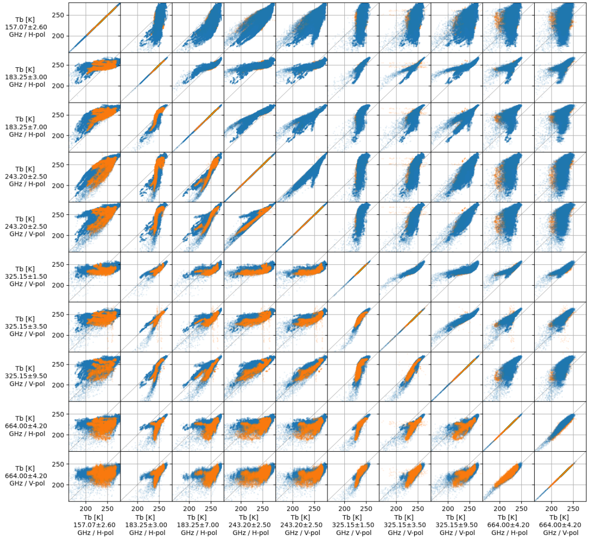
Figure 16: Scatter plots of simulated (blue dots) and actual ISMAR and MARSS observations (orange dots) for data from ten channels, and for a flight altitude around 9.4 km, and an observation zenith angle of 140^\circ . The simulation is not performed to match each actual observation individually. See text for more details.
