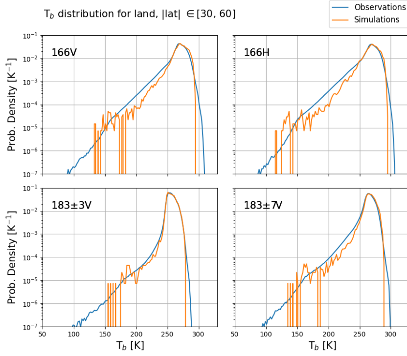
Figure 32: Brightness temperature ( T_b ) probability distributions for each of the high-frequency channels of GMI for land at mid-latitudes i.e. only data from latitudes -60 to -30 and 30 to 60 are included.
