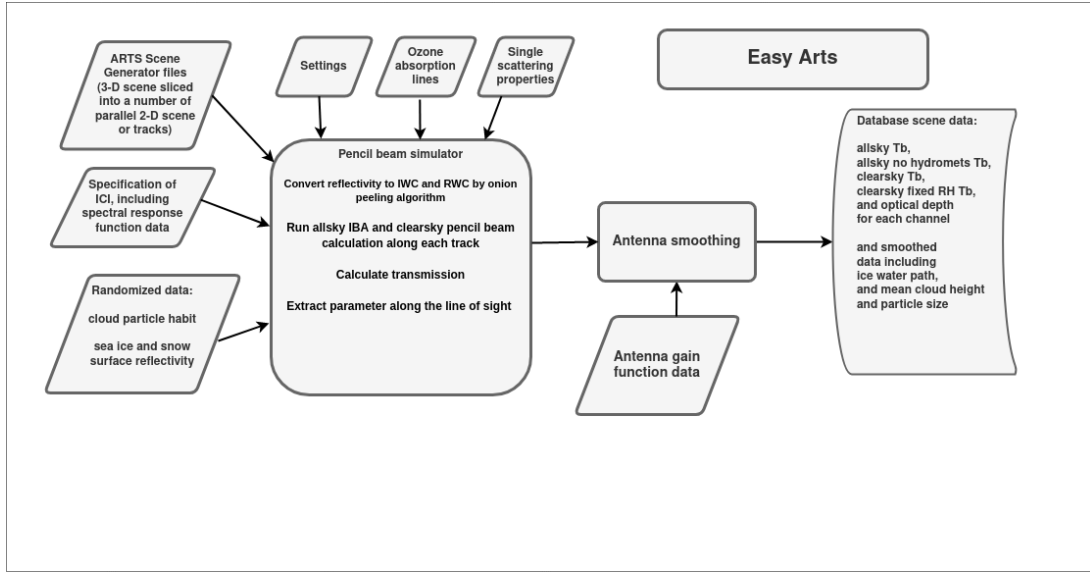
Figure 3: Flowchart summarising the input data, processes, and outputs of the scheme developed for the ICI simulation.
