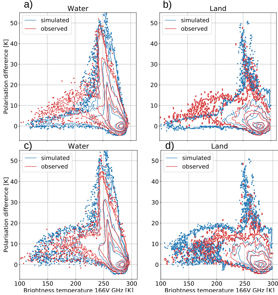
Figure 6: Polarisation difference contours ( 166V-166H ) as a function of 166V GHz brightness temperatures ( T_b ) for observed GMI data (red) and simulated values (blue) for water and land. In (a) and (b) the simulations assume hydrometeors to have TRO, while in (c) and (d) the ARO effects are simulated using a scheme similar to Barlakas et al. (2021).
