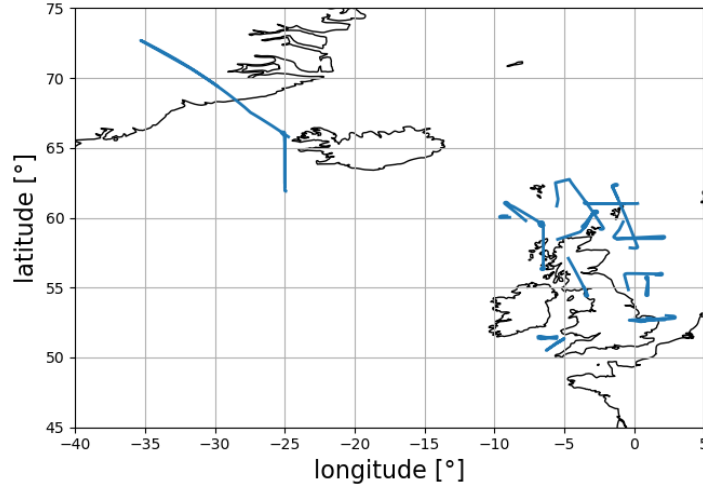
Figure 15: Flight tracks of the FAAM BAe-146 research aircraft where ISMAR and MARSS observations are available and flight altitude is above 9 km.
