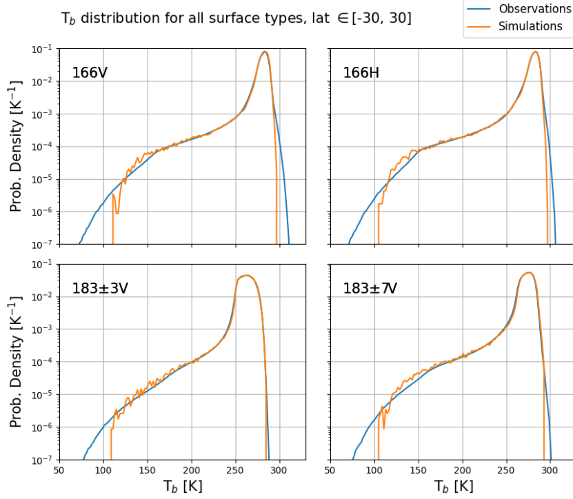
Figure 29: Brightness temperature ( T_b ) probability distributions for each of the high-frequency channels of GMI for all surface types at tropical latitudes, i.e. only data from latitudes -30 to 30 are included.
