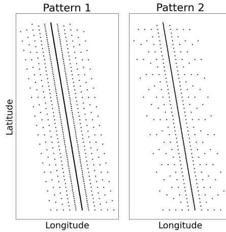
Figure 21: Patterns 1 and 2. Both patterns consist of the same tracks, but pattern 2 has double the amount of spacing between points as pattern 1. Patterns 5 and 6 differ from patterns 1 and 2, respectively, by the removal of the two outermost tracks.
