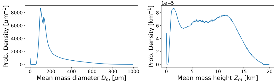
Figure 2: Probability density functions (PDF) of D_m and Z_m values present in the database. The peaks in probability density arising at D_m = 0 \mu\text{m} and Z_m = 0 \text{ km} corresponds to cases in which IWP = 0 \text{ kg m}^{-2} .
