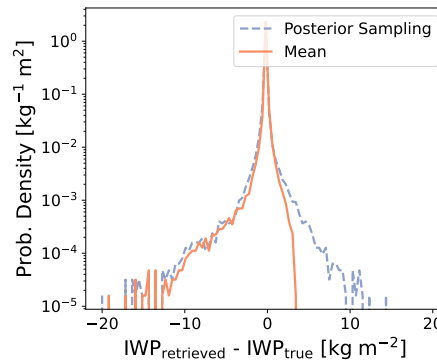
Figure 13: PDF of retrieval error. Distributions are shown using mean as the point estimate of IWP and using samples from the a posteriori distribution as the point estimate.
