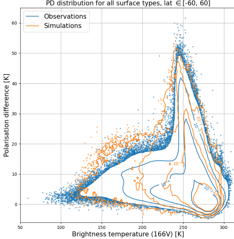
Figure 10: Joint probability distributions of polarisation difference (PD) and brightness temperature for the 166V channel ( T_{b,166V} ) are plotted for all surface types and latitudes in the range -60 degrees to 60 degrees. PD is defined as T_{b,166V} - T_{b,166H} and details of the modelling of hydrometeors in the simulations can be seen in Sec. 3.4 in the Task2 report. Contour lines of the probability distributions for observations (blue) and simulations (orange) are seen at levels 10^{-6} \text{ K}^{-2} , 10^{-5} \text{ K}^{-2} , 10^{-4} \text{ K}^{-2} and 10^{-3} \text{ K}^{-2} . A random sample of 1% of the simulated data points with lower probability than 10^{-6} \text{ K}^{-2} are plotted as blue dots. For the simulations all point with lower probability than 10^{-6} \text{ K}^{-2} are plotted as orange dots.
