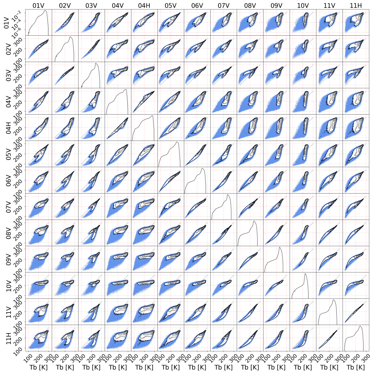
Figure 5: PDFs of simulated antenna-weighted brightness temperatures T_b in a version of the retrieval database consisting of \sim 8.9 \times 10^6 cases. On the diagonal, 1-dimensional PDFs are shown. Two-dimensional joint distributions are shown off-diagonal. Contour lines correspond to [10^{-1}, 10^{-2}, 10^{-3}, 10^{-4}, 10^{-5}, 10^{-6}] K^{-2} , with 10^{-5} K^{-2} corresponding to the outermost contour line. Samples that occur with a probability density less than 10^{-6} K^{-2} are represented by blue markers.
