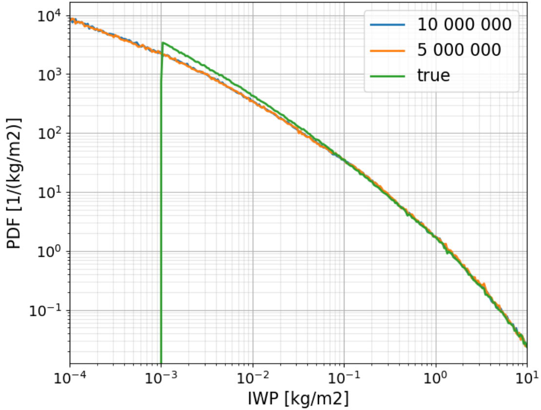
Figure 27: Retrieved (posterior median value) and true probability density function of IWP, for the data displayed in Figure 26.
