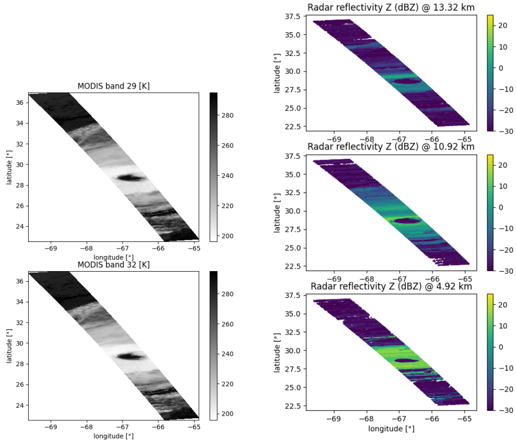
Figure 9: ‘Barkerized’ data for the scene shown in Figure 8. The left panels show Modis band 29 and 32 data extending \pm 50 km in the across-track direction of CloudSat sub-satellite path. The right panels show constructed 2-D cross-sections of radar reflectivity at three different altitudes.
