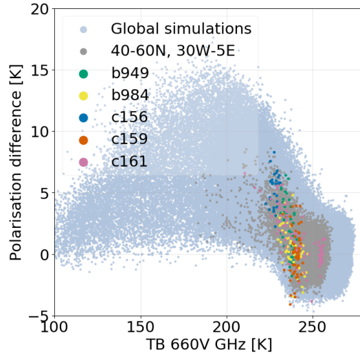
Figure 7: The scatter plot showing the PD vs Tb_V at 660 GHz. The light blue dots are for near global simulations; the gray dots denote simulations in 40^\circ\text{N} - 60^\circ\text{N}/30^\circ\text{W} - 5^\circ\text{E} . The five alphanumeric codes depict observations from five flight campaigns as described by Fox (2020).
