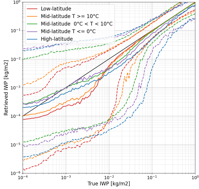
Figure 20: Estimated retrieval performance for IWP and five climatic regions. The solid lines show the median of the retrieved posterior median values, and the dashed lines show the median of the retrieved 5th and 95th percentile.
