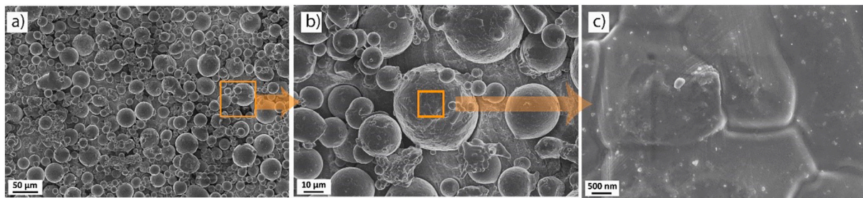
Fig. 1. Morphology of virgin powder at different magnifications observed through HR-SEM.
