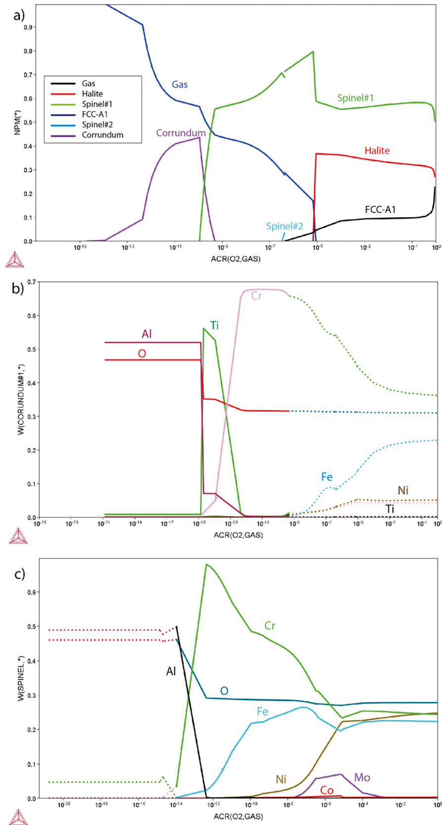
Fig. 11. Thermodynamic calculations using Thermo-Calc 2021: (a) equilibrium phase fraction at 1500 °C with varying oxygen partial pressure, (b) composition of corundum 1 phase, and (c) composition of spinel phase. The dashed lines correspond to the elemental compositions in the metastable phase.
