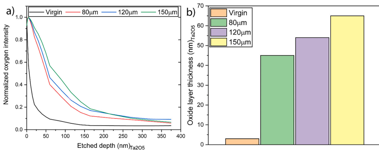
Fig. 10. A comparison of a) normalized oxygen intensity w.r.t. etched depth and b) oxide layer thickness of feedstock powder and the spatter samples gathered at 80 µm, 120 µm, and 150 µm layer thickness.
