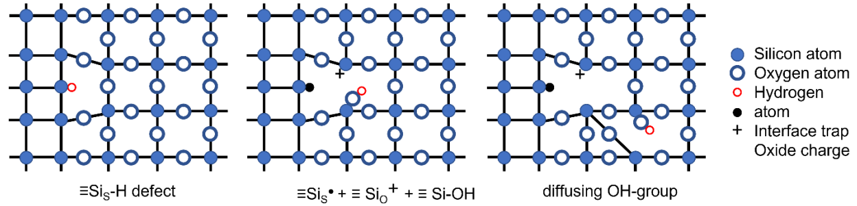
Fig. 3. Schematic two-dimensional representation of the Si-SiO 2 interface showing a) the Si-H defect, b) electrical activation of the \equiv\text{Si}_\text{S}\text{-H} defect during negative-bias stress forming an interface trap ( \bullet ), an oxide charge (+), and a hydroxyl (OH) group that c) may diffuse in the oxide and be the reaction-diffusion-limited factor. ( \equiv\text{Si}_\text{S} indicates a silicon atom bonded to three other silicon atoms while \equiv\text{Si}_\text{O} indicates a silicon atom bonded to three oxygen atoms.) 5
