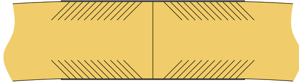
Figure 2.7: Illustration of the moment resisting joints made of inclined self-tapping screws and steel plates for the arch of the University Sport Hall (Singapore)
