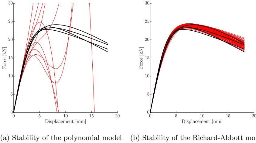
Figure 4.6: Stability of the models. In black are experimental curves, in red the realizations of the models
