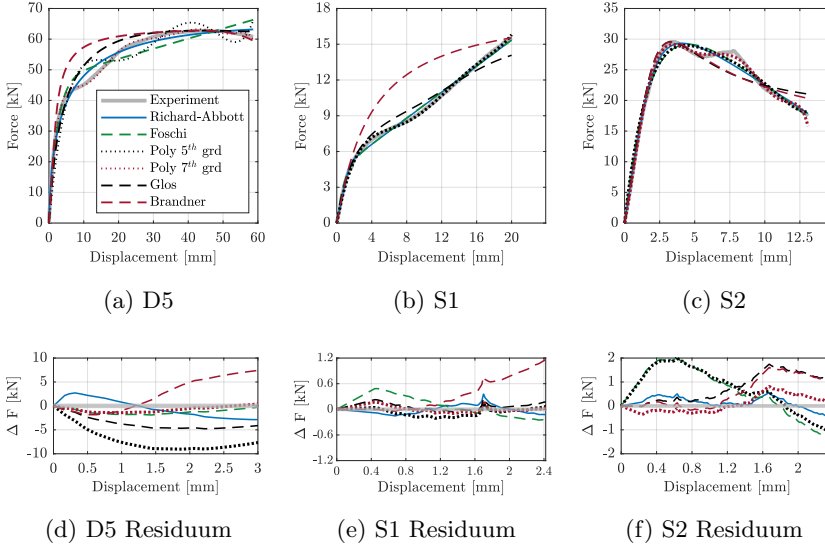
Figure 4.5: Application of parameterization equations to different types of experimentally determined slip curves.
