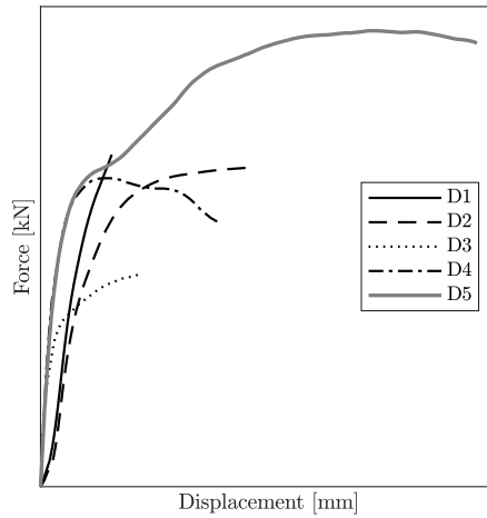
Figure 2.16: Typical load-displacement curves of joints with dowel [65], [66]
