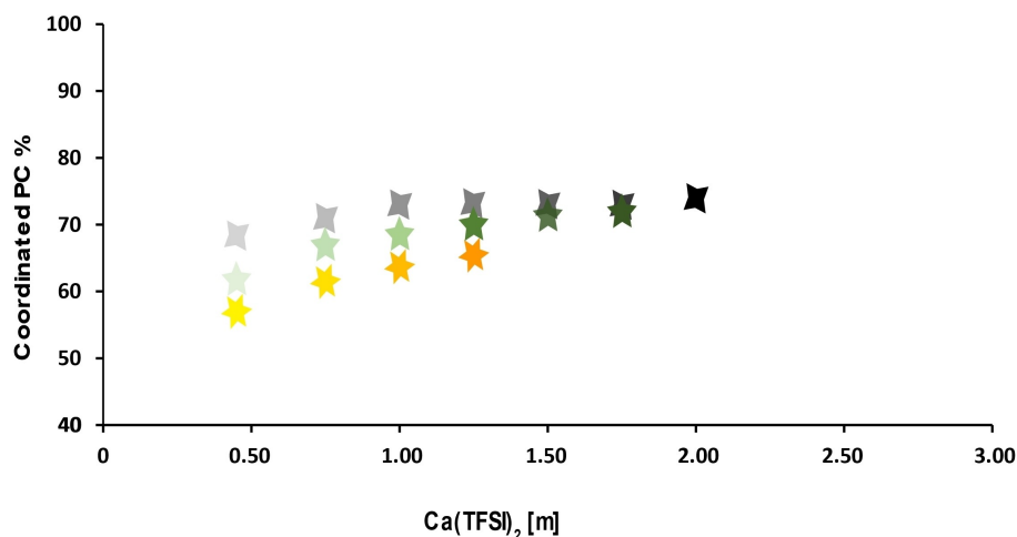
Figure 12. The cation-solvent interactions as function of nominal and local salt concentration, with the symbols corresponding to the latter: \blackstar 2.50 m, \star 2.00 m, and \blackstar 1.50 m.
